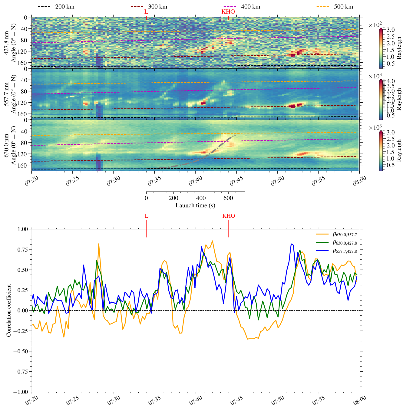
Figure 7. The top figure shows the MSP data just before and after the 07:34 UT launch. The vertical blue stripe is due to clearing of snow from the slit. L and KHO mark the launch and passing east of KHO , respectively. Dashed lines represent the sunlit part of the atmosphere, with everything south of the line being sunlit at and above that altitude. Sunlit means that the light from the Sun has not passed below 150 km in order to get to the point of interaction. In the 630.0 nm figure the dashed and dotted gray line represents the rocket track mapped to the MSP field of view at a height of 240 km. The bottom figure shows the correlation coefficients for the time around the launch at 07:34 UT based on the data in the top figure.
