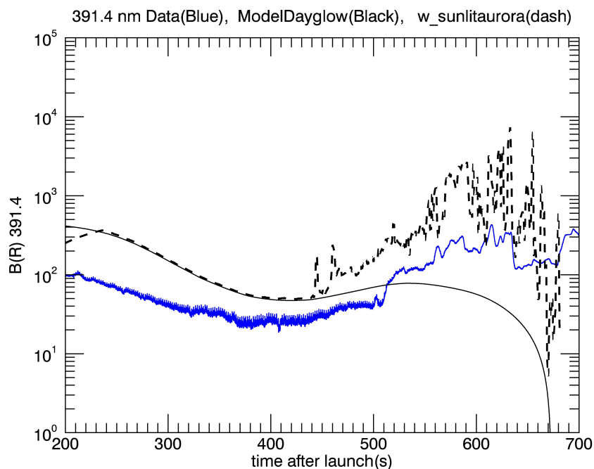
Figure 6. A plot of the brightness in Rayleighs of the emission from the (0,0) band of the N_2^+ 1NG system at 391.4 nm from the RENU2 blue photometer vs time after launch. Also shown is the model dayglow data (solid line) and the dayglow plus the emission due to the auroral precipitation (see text). 200 s corresponds to 07:37:30 UT and 700 s to 07:45:40 UT.
