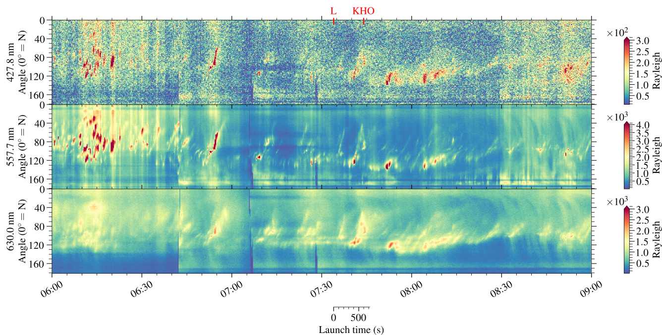
Figure 2. The MSP data from 6 UT to 9 UT. It shows the three recorded wavelengths over the North to South scan along the magnetic meridian. The vertical dark blue stripes are from when the slit covering the MSP was cleaned of snow. L and KHO mark the launch and passing east of KHO.
