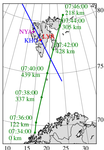
Figure 1. Figure showing the ground track for the RENU2 rocket, green, and the Meridian Scanning Photometer (MSP) scan line, blue, when scanning above 20^\circ elevation angle. The location of Longyearbyen (LYR), Ny-Ålesund (NYA) and the Kjell Henriksen Observatory (KHO) are shown.
