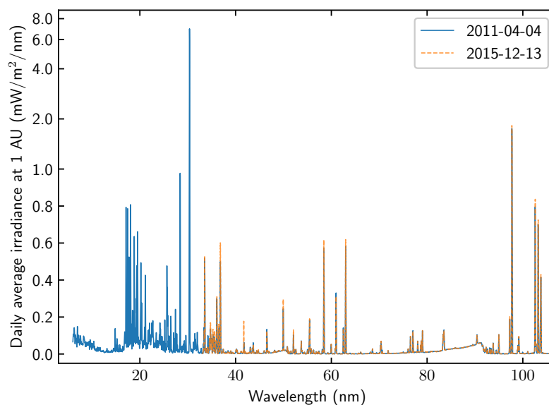
Figure 3. Measurements of daily average irradiance at 1 AU from the EVE instrument from the day of the launch 2015-12-13 (orange) and the closest match to the launch day from when the MEGS-A detector worked (blue). Notice that the irradiance scale is linear below 1 \text{ mW/m}^2/\text{nm} and logarithmic above.
