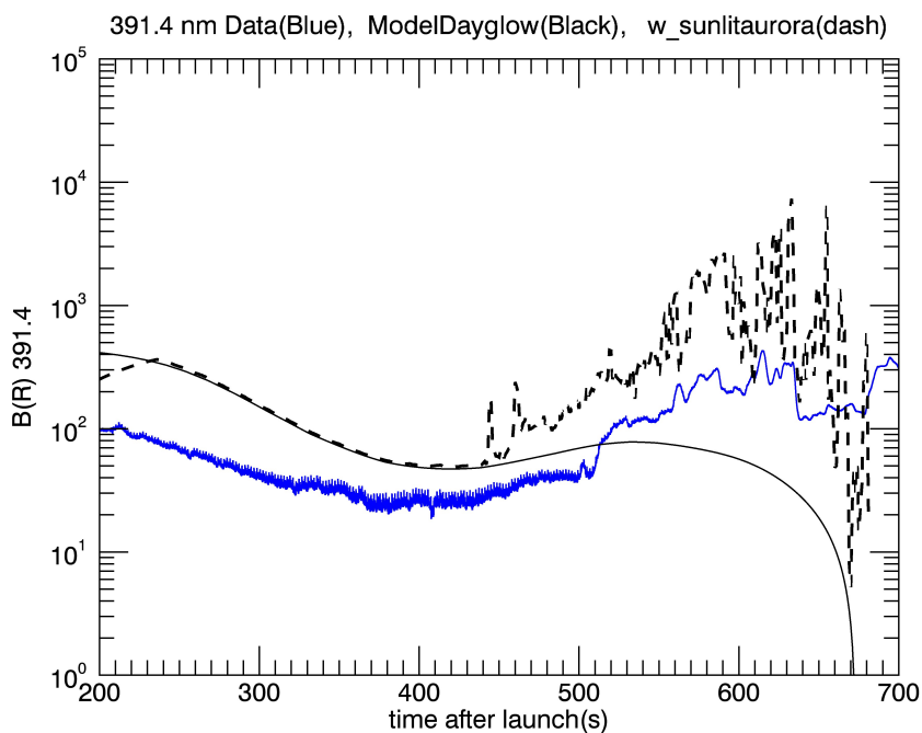
Figure 6. A plot of the brightness in Rayleighs of the emission from the (0,0) band of the N_2^+ 1NG system at 391.4 from the RENU2 blue photometer vs time after launch. Also shown are the Strickland model predictions (see text) for the N_2^+ 1NG system at 391.4nm dayglow (solid line) and for the N_2^+ 1NG system at 391.4 dayglow plus the N_2^+ 1NG system at 391.4 emission due to the auroral precipitation. A time after launch of 200 corresponds to 07:37:30 UTC while 700 corresponds to 07:45:40 UTC.
