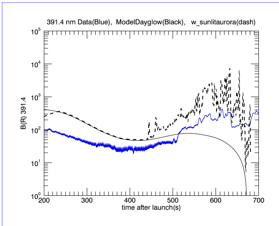
Figure 6. A plot of the brightness in Rayleighs of the emission from the (0,0) band of the N_2^+ ING system at 391.4 nm from the RENU2 blue photometer vs time after launch. Also shown are the Strickland model predictions (see text) for the N_2^+ ING system at 391.4 nm dayglow (solid line) and for the N_2^+ ING system at 391.4 nm dayglow plus the N_2^+ ING system at 391.4 nm emission due to the auroral precipitation. A time after launch of 200 s corresponds to 07:37:30 UTC while 700 s corresponds to 07:45:40 UTC.
