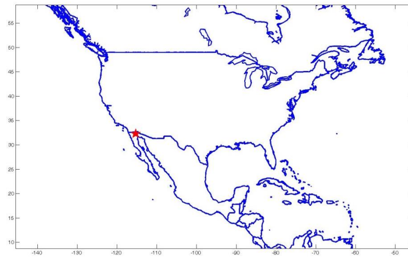
Fig.3 The location of 2010 M_w 7.2 Mexico earthquake
