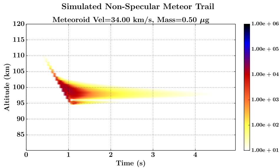
Figure 9. Simulation showing the effects of neutral wind shears, using a meteoroid with a mass of 0.5 \mu\text{g} that is traveling at 34 \text{ km/s} . The background atmosphere/ionosphere conditions have a vertical profile similar to those displayed in Figure 5.
