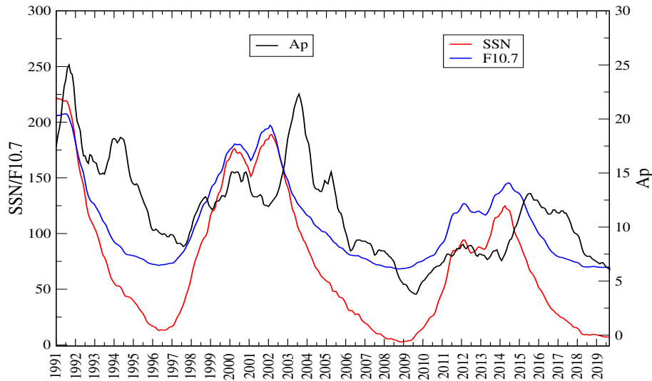
Figure 2. Monthly smoothed values of archived Sun Spot Number (SSN), Radio solar flux (F10.7) and geomagnetic Ap from January 1991 - March 2020 (updated predicted data in Nwankwo and Chakrabarti (2013) with actual data).
