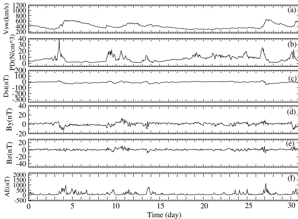
Figure 3. 1-hour averaged variations in V_{sw} , PD, Dst, IMF B_y and B_z , and AE for the geomagnetically quiet, solar minimum interval 1-31 July 2006.
