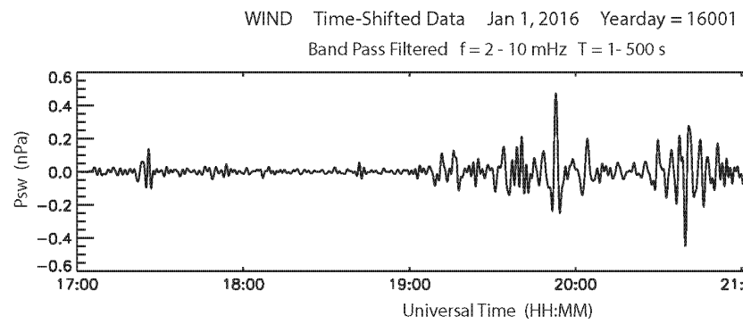
Figure C. Wind time-shifted filtered data in the band of frequencies from 17:00 UT to 22:00 UT on January 1, 2016.
