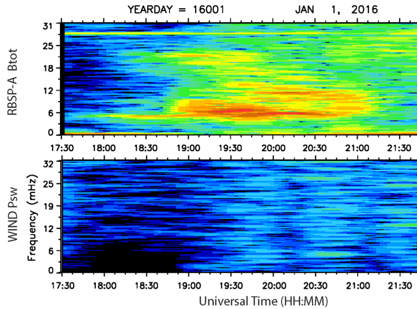
Figure B. Dynamic spectra of the RBSP-A total magnetic field strength and solar wind pressure from 17:30 UT to 22:00 UT on January 1, 2016.
