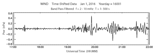
Figure C. Wind time-shifted filtered data in the band of frequencies from 2 to 10 mHz from 17:00 UT to 22:00 UT on January 1, 2016.
