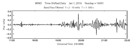
Figure C. Wind time-shifted filtered data in the band of frequencies from 2 to 10 mHz from 17:00 UT to 22:00 UT on January 1, 2016.
