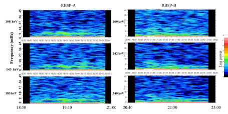
Figure A. Dynamic spectra for electrons with selected energies observed by RBSP-A from 18:30 to 21:00 UT and by -B from 20:40 to 23:00 UT on January 1, 2016.
