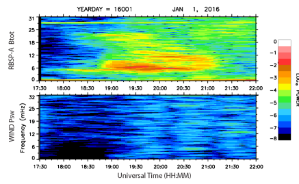
Figure B. Dynamic spectra of the RBSP-A total magnetic field strength and the WIND solar wind pressure from 17:30 UT to 22:00 UT on January 1, 2016.
