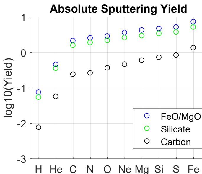
Figure 2. Sputtering yield for \text{Fe}_{0.4}\text{Mg}_{0.6}\text{O} (blue), silicate (green) and carbon (black) as a function of solar wind ion composition and its mean speed (yields for slow SW conditions are given).
