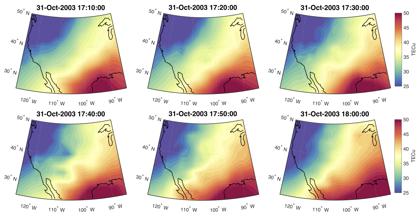
Figure 4. Series of vTEC from the MIDAS GPS inversion. Each frame is separated by 10 minutes.
