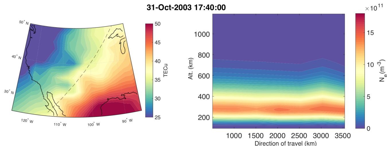
Figure 5. (Right) NE-SW cross-section of the full inverted electron density, and (left) the path of the placement of the cross-section in the vTEC map.
