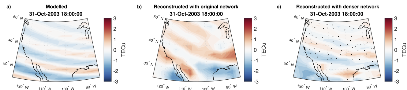
Figure 8. a) The modelled LSTID vTEC a and filtered inversions from the simulated data (b) and c). c) uses a denser network than the real inversion, where the receiver locations of the network are indicated with black markers.
