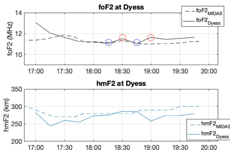
Figure 6. foF2 (top) and hmF2 (bottom) observations for the Dyess ionosonde ( 32.4^{\circ}\text{N} , 99.8^{\circ}\text{W} ) and MIDAS equivalent sampled at the same location on 31 October 2003.
