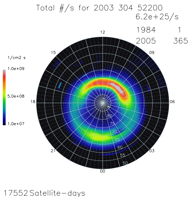
Figure 9. OVATION particle flux for 31 October 2003 at 14:30 UTC.
