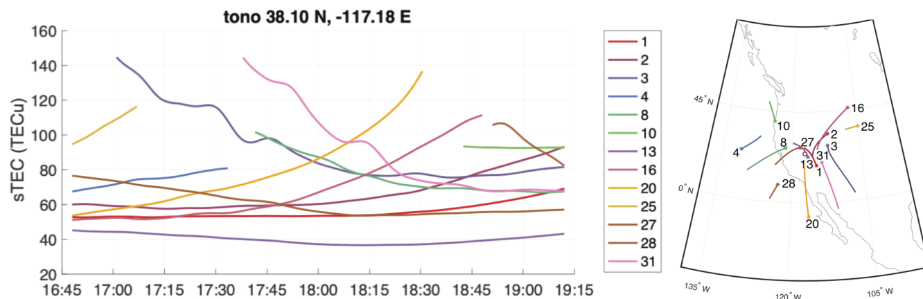
Figure 3. Biased sTEC from GPS receiver station tono on 31 October 2003.
