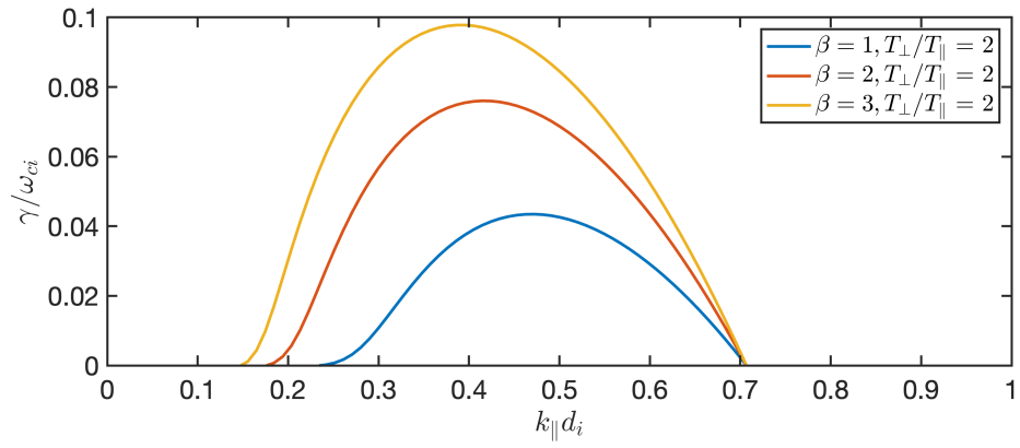
Fig. 1. Growth rate of the proton cyclotron instability for three different beta plasma, computed with HYDROS
