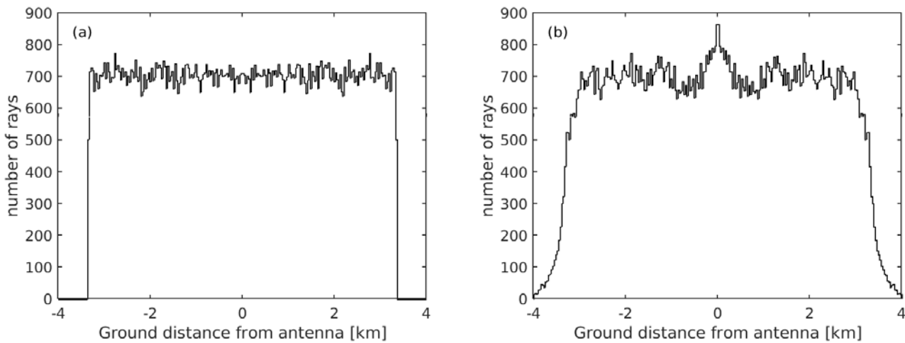
280 Figure 5. Histograms of the number of rays arriving on the ground from 600 km, for (a) when no irregularities are present and (b) after propagating through irregularities having parameters A = 1 \times 10^{-6} , W = 50 m, and L = 80 km. The bin width is 32 m, equal to the antenna diameter. There is a clear enhancement in the number of rays arriving at the antenna at 0 km. In the final modelling shown in Figs. 6-9 an extra condition is imposed on the number of rays arriving within the 32 m bin at 0 km, namely that each ray is within the beam width of approximately \pm 0.35^\circ .
