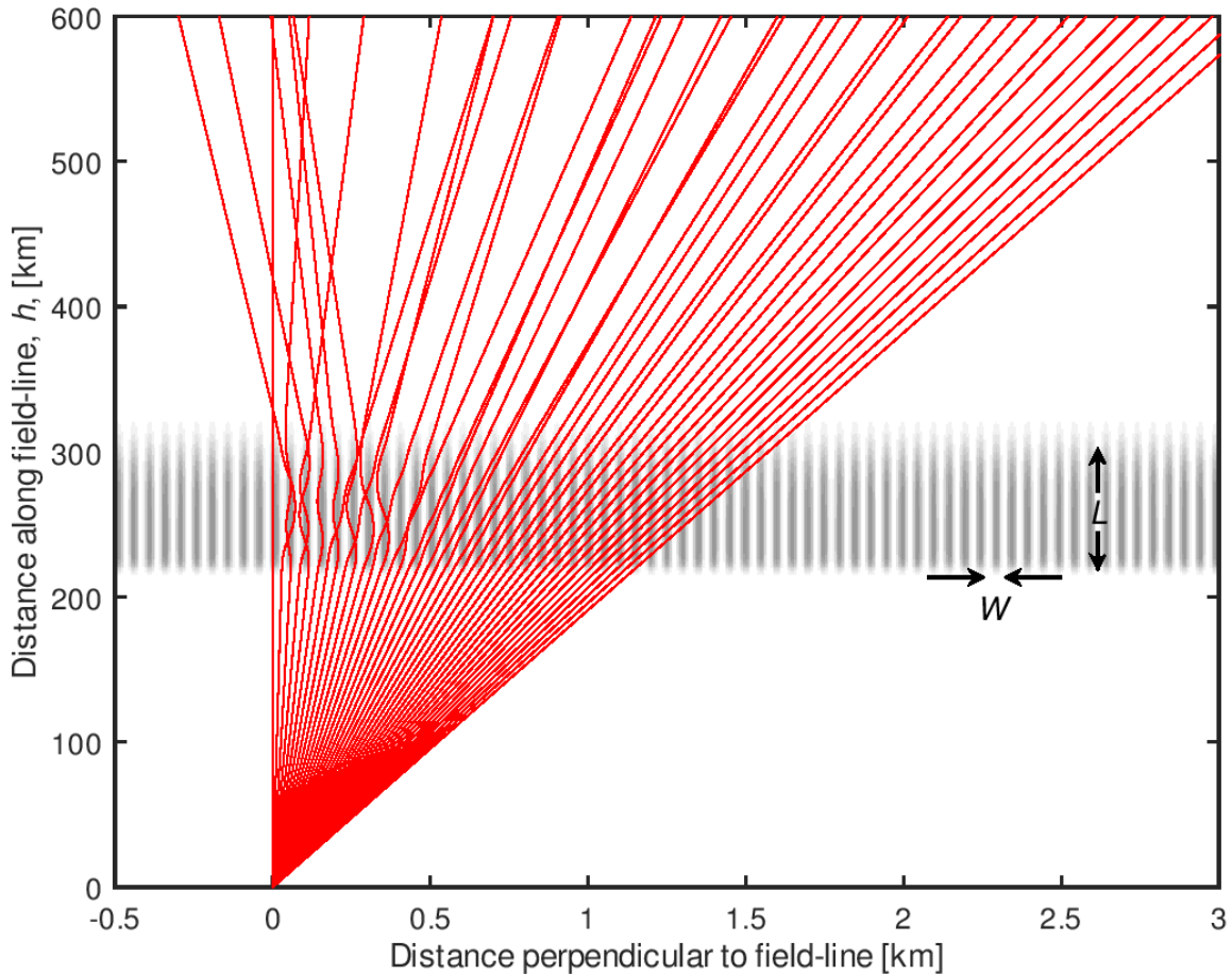
Figure 2. Ray paths of a set of 40 up-going 933 MHz waves from the transmitter at (0,0) with launch zenith angles evenly spaced between 0^\circ and 0.3^\circ passing through a region of vertically aligned irregularities, shown in grey shading, with A = 1 \times 10^{-6} , W = 50 m and L = 80 km between 220 and 300 km. The magnetic field lines are assumed to be vertical. These rays illustrate the effects of refraction, but in the final modelling we use 3333 realistically spaced rays both sides of zenith to represent the transmitted beam.
