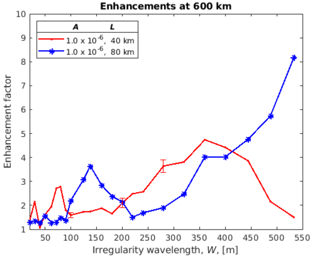
330 Figure 9. Enhancement factors for 933 MHz backscatter from 600 km for two lengths of the irregularity, L , along the field line for a fixed irregularity depth, A .
