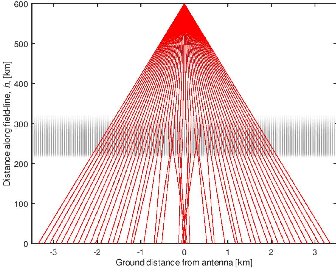
Figure 3. Backscattered down-going 933 MHz rays from one up-going ray which arrived at 600 km. The 51 rays pass through the same region of irregularities as in Fig. 2 with A = 1 \times 10^{-6} , W = 50 m and L = 80 km between 220 and 300 km. There is a clear increase in the density of rays, or backscattered power, near the receiver antenna at (0,0), as well as regions of weaker backscatter further away.
