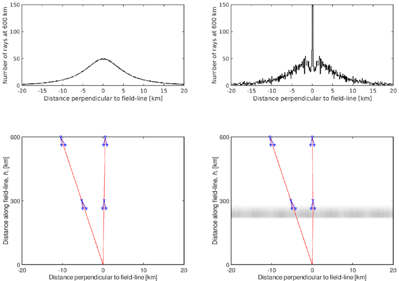
255 Figure 4. Schematic diagram of the model showing (in red) two out of thousands of rays launched from the transmitter at (0,0), for the free-space case on the left and with irregularities (in grey) on the right. The zenith angles of these two rays are -1^\circ and 0.05^\circ . The histograms at the top show the distribution of rays arriving at 600 km. In the modelling, a fan of 30 rays is re-launched from each incoming ray at two heights of 300 and 600 km as depicted by the blue downward arrows which show the edges of the fan at \pm 0.32^\circ about the incoming ray direction. The ratio of the number of rays arriving on the ground within \pm 16 m of (0,0) and within \pm 0.35^\circ of the vertical field line for the case with irregularities to that without is a measure of the 260 backscatter enhancement measured by the radar.
