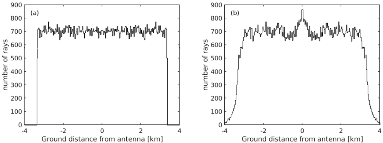
275 Figure 5. Histograms of the number of rays arriving on the ground from 600 km, for (a) when no irregularities are present and (b) after propagating through irregularities having parameters A = 1 \times 10^{-6} , W = 50 m, and L = 80 km. The bin width is 32 m, equal to the antenna diameter. There is a clear enhancement in the number of rays arriving at the antenna at 0 km.
