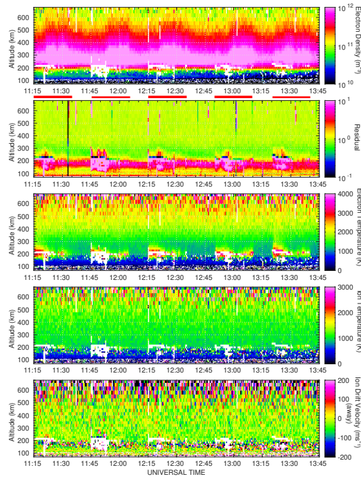
Fig. 1. An example of wide altitude ion line enhancements (WAILE). The top panel shows the enhancements interpreted by the analysis as an electron density increase between about 200 km and 600 km. The HF on t
