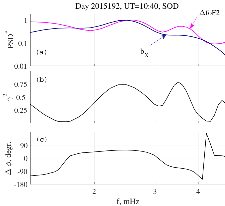
Figure 7. Spectral parameters for the event 2: (a) normalized PSD spectra of \Delta\text{foF2} and b_X pulsations, (b) spectral coherence; (c) phase difference.
