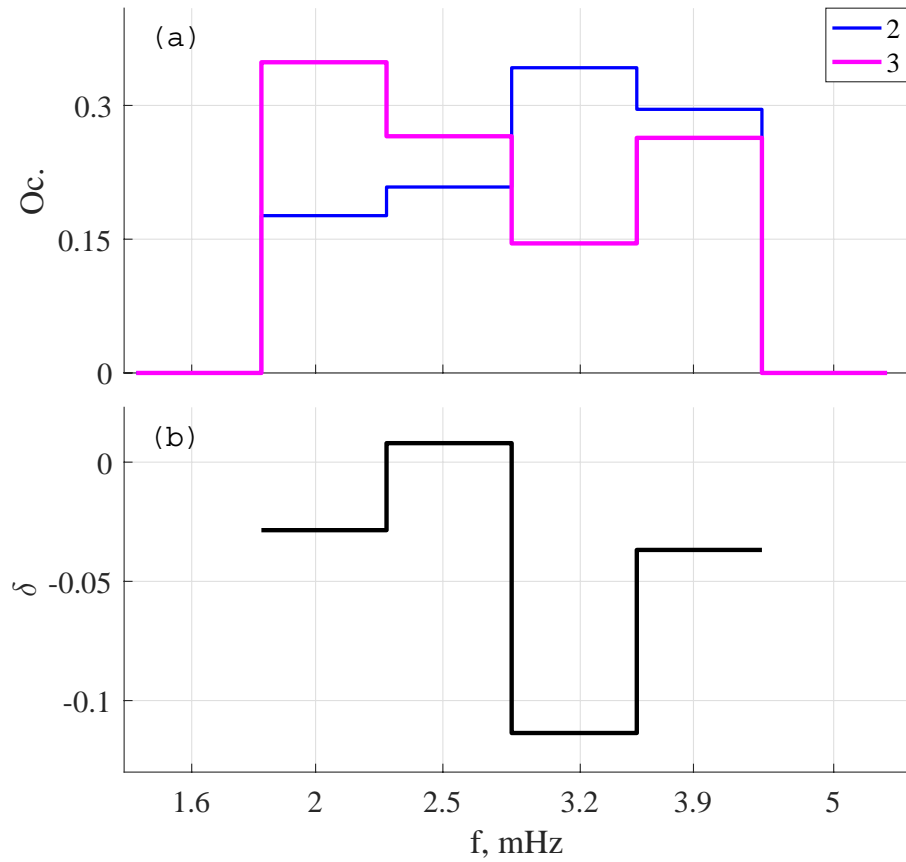
Figure 10. Frequency histogram, for b_X (group 2) and \Delta\text{foF2} (group 3) fluctuations (a) and for the parameter \delta = \log(\Delta_{f2,0}/\Delta_{f2,R}) , where \Delta_{f2,0} and \Delta_{f2,R} are the mean values of \Delta_{f2} for simultaneous and random intervals (b).
