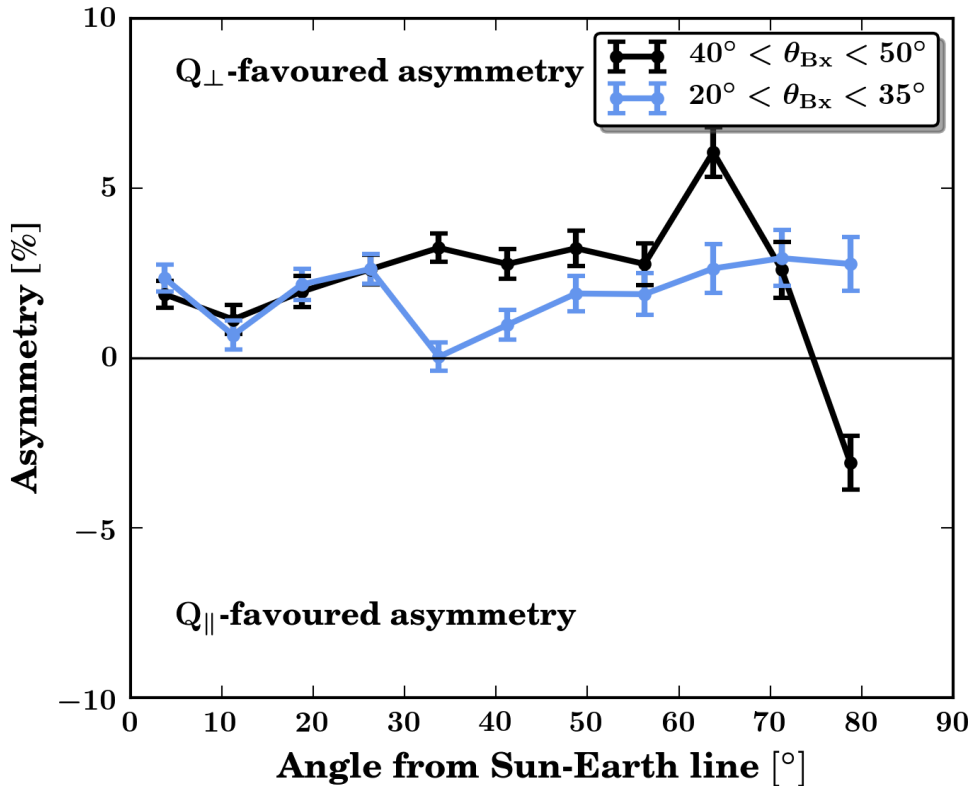
Fig. 2. Magnetic field asymmetry in the central magnetosheath (observations) (Fig. 7a in the manuscript)
