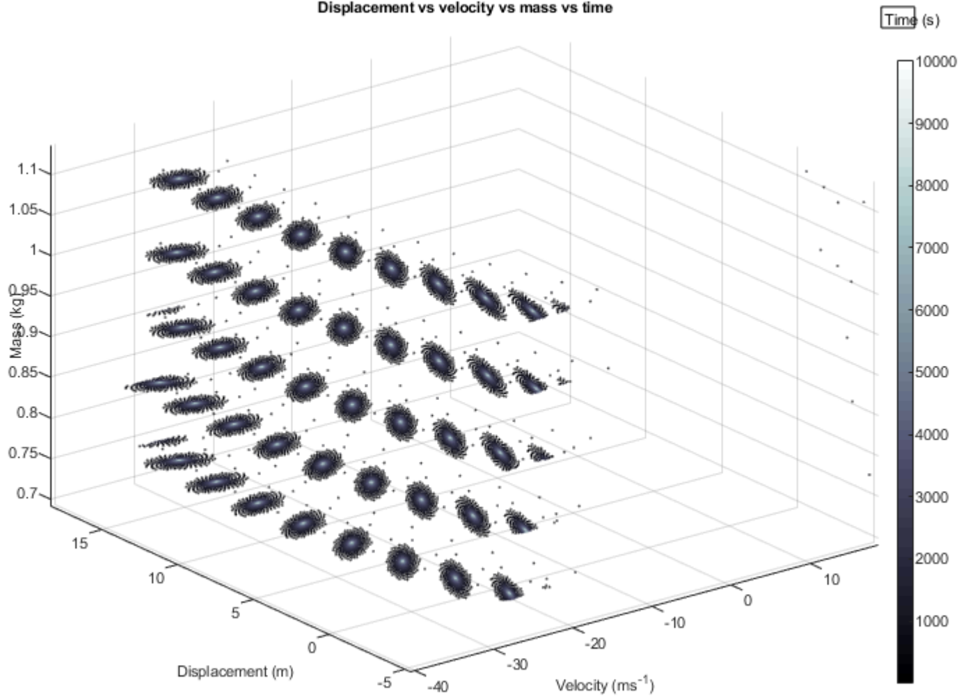
Planetary Magnetotail Dynamics Model: Displacement vs velocity vs mass vs time
