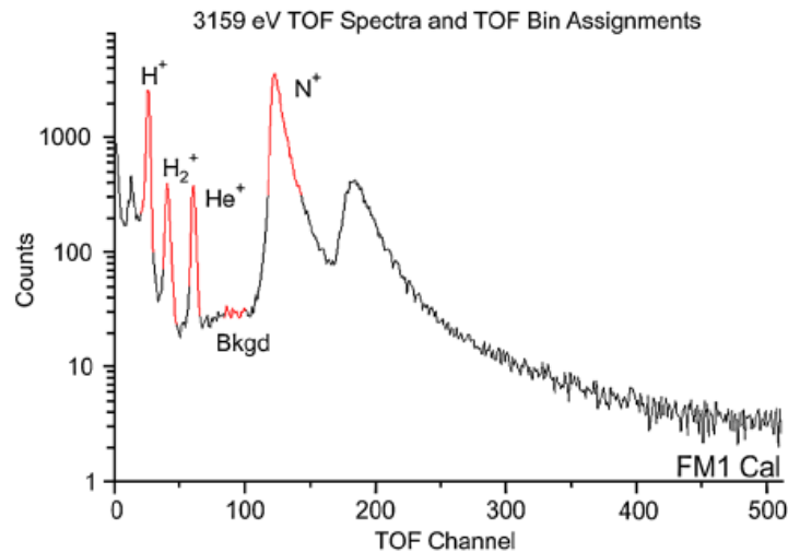
Fig. 20 TOF spectrum for four ion species and background ( H_2^+ is a substitute for He^{++} and N_2^+ is a substitute for O^+ ). Red areas demarcate bins that define ion species and background. The peak at \sim 200 ns corresponds to N_2^+
