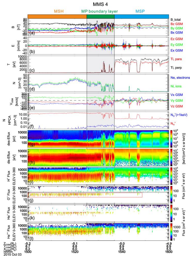
Fig. 2. Fig.2 The energetic \text{O}^+ is observed at the magnetopause during an intense substorm on 03 October 2015 by MMS 4.
