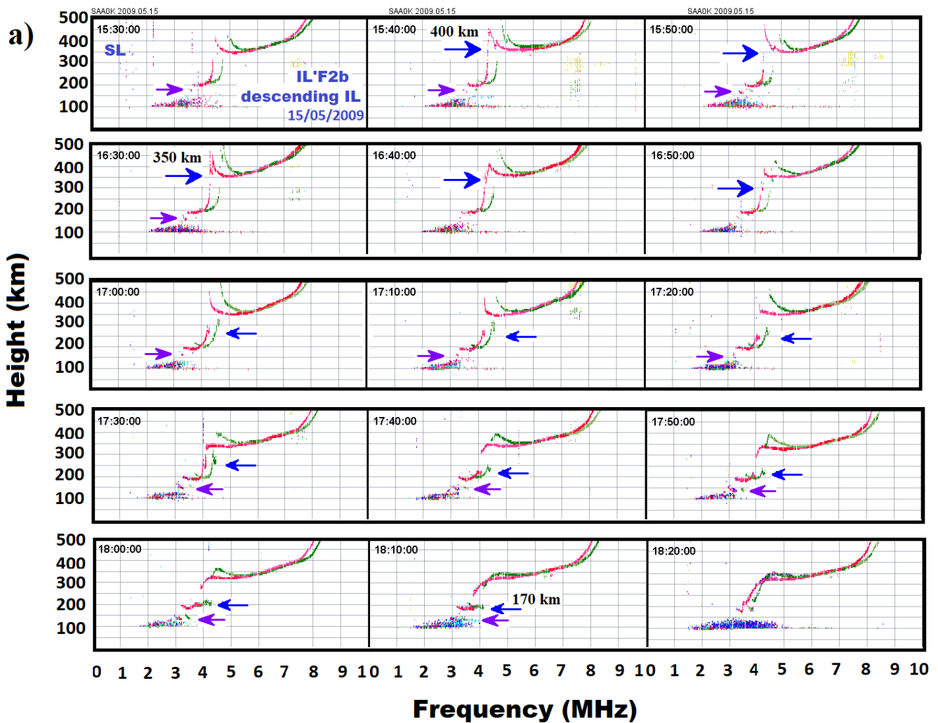
FIGURE 10: a) Sequence of ionograms during 1530 – 1820 UT on 15 May 2009 showing the perturbation in the F2 layer trace that reached low altitudes and evolved to a descending intermediate layer over São Luís. The blue arrow indicates the downward movement of perturbation in F layer and the purple arrow indicates the presence of another IL occurring
