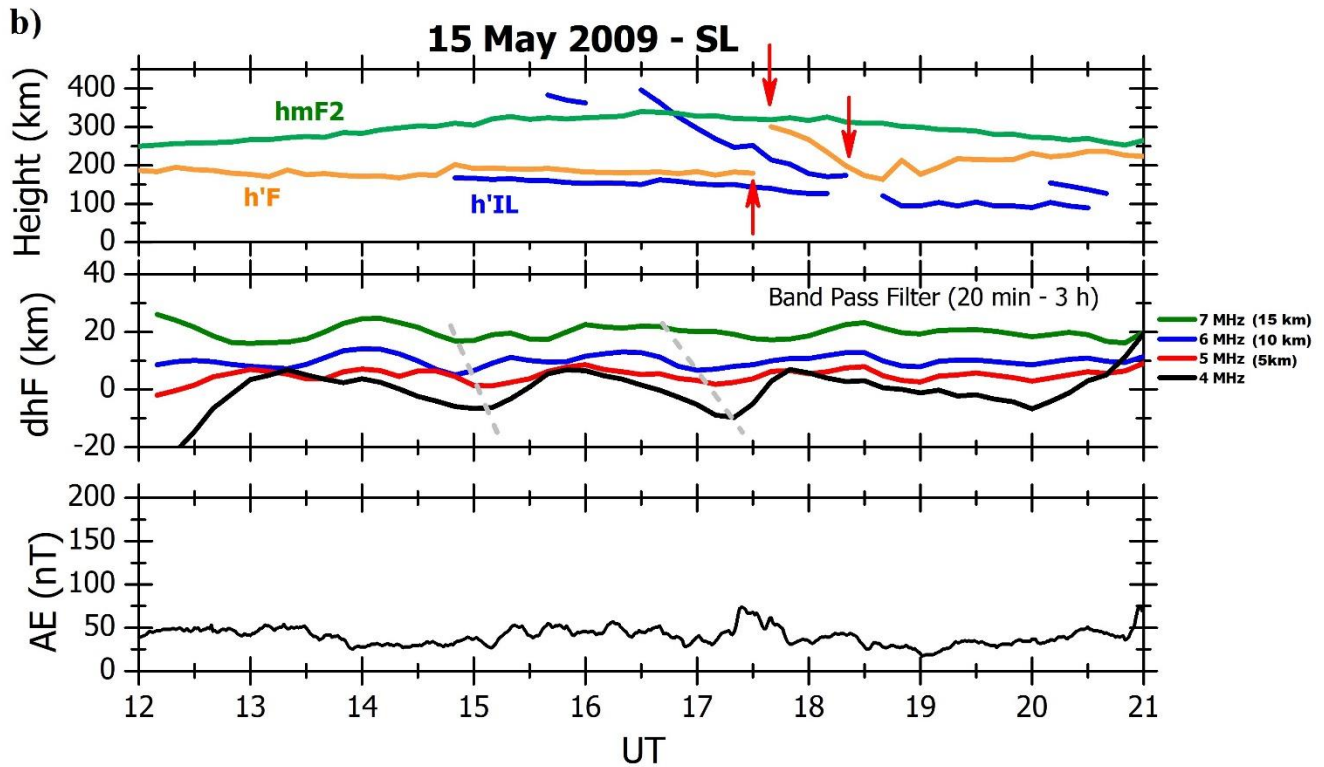
FIGURE 10: b) The virtual height of the F layer h'F (orange line), the F2 layer peak hmF2 (green line) and the virtual height of ILs ( h'IL , blue line). The red arrows indicate some modifications in the F layer in the form of the formation of the IL from a detachment of the F1 layer and the junction of the IL with the F1 layer. The middle panel shows the Band-pass filtered (for 20 min. to 3h periods) height oscillations at frequencies 4, 5, 6 and 7 MHz, displaced cumulatively by 5 km at each frequency. The downward phase propagation is indicated by the dashed gray line. The last panel shows the auroral activity.
