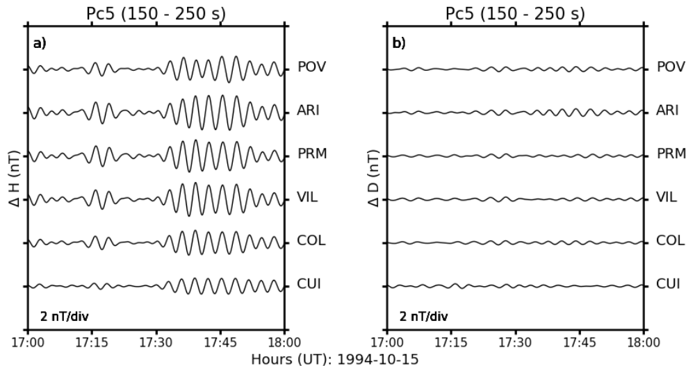
Figure 4. The same as Figure 3, for Pc5 pulsations in the afternoon on October 15, 1994. An event is observed in the H-component after 1730 UT.
