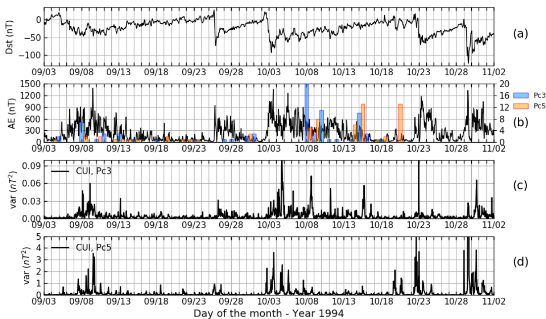
15 Figure 2. Geomagnetic indices and filtered ground geomagnetic pulsations during the period September 3 to November 1, 1994. (a) Dst index; (b) AE index with the temporal location and number of events chosen for the pulsation analysis; (c) variance of Pc3 pulsations in the H-component of the CUI station; (d) variance of Pc5 pulsations in the H-component of the CUI station.
