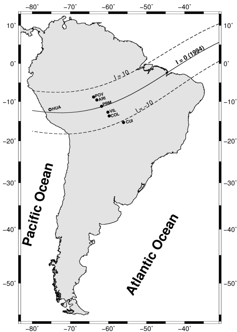
10 Figure 1. Geographic location of the six geomagnetic stations in South America and contours of the geomagnetic field at 1994. The solid line shows the dip equator ( I = 0^\circ ), and the dashed lines represent \pm 10^\circ inclination angles. Location of the Huancayo station (HUA) is also indicated. Geomagnetic field values were obtained from the IGRF model.
