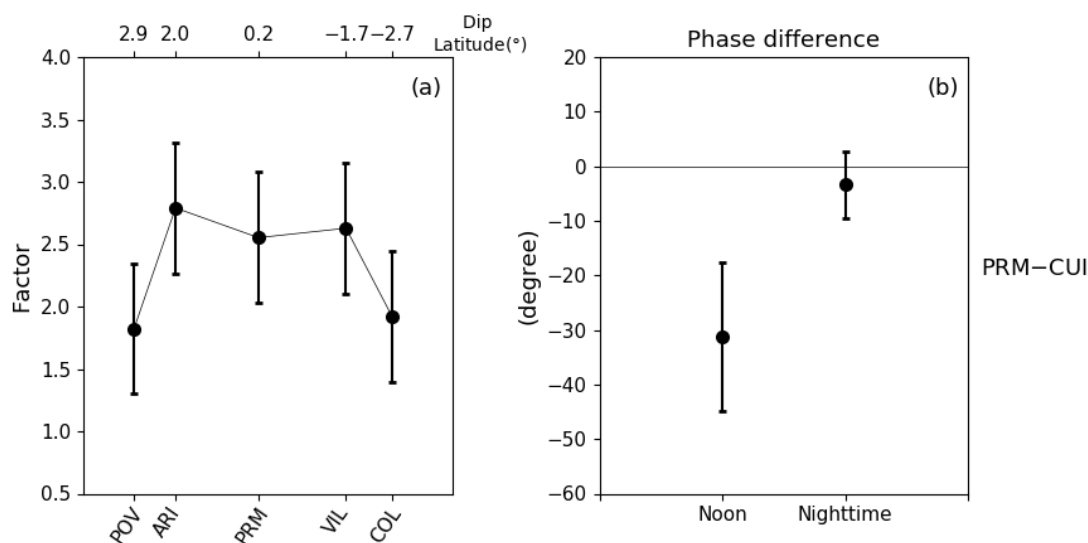
15 Figure 8. (a) Latitudinal profile of amplification factors for Pc5 pulsations around noon. (b) Phase delays between the dip equator station (PRM) and off-equatorial station (CUI) for Pc5 events during nighttime and around noon. Mean and standard deviations are indicated by dots and bars, respectively.
