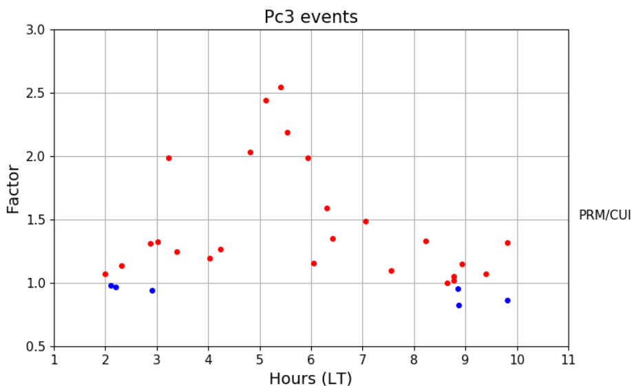
Figure 10. Distribution of Pc3 relative amplitudes (PRM/CUI) in H-component between 2 and 10 LT. In red are values greater than one (amplification) and in blue are values less than one (damping).
