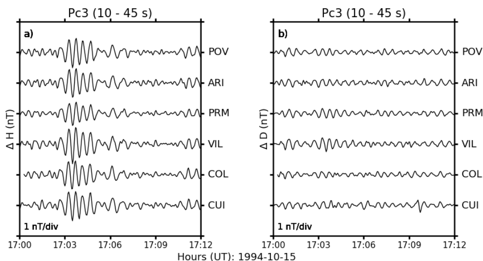
Figure 3. Band-pass-filtered geomagnetic variations (H and D components) in the Pc3 interval, shortly after noon on October 15, 1994. A Pc3 event starting at ~1703 UT is observed.
