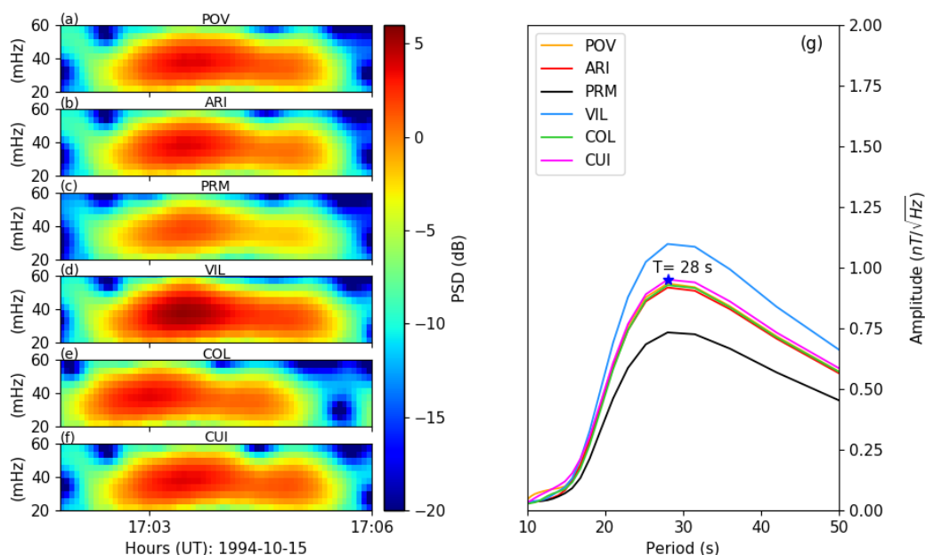
Figure 5. Power spectral analysis for the Pc3 pulsation on October 15, 1994 shown in Figure 3. Left panels (a-f) show dynamic spectrograms of power spectral density during the event. Right panel (g) shows the average spectral amplitude at each station with identification of the period of peak amplitude in CUI station.
