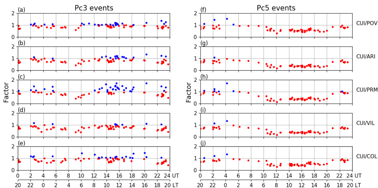
Figure 6. Local time dependence of occurrence distributions of Pc3 and Pc5 relative amplitudes at the equatorial stations. In blue are values greater than one (damping), in red are values less than one (amplification).
