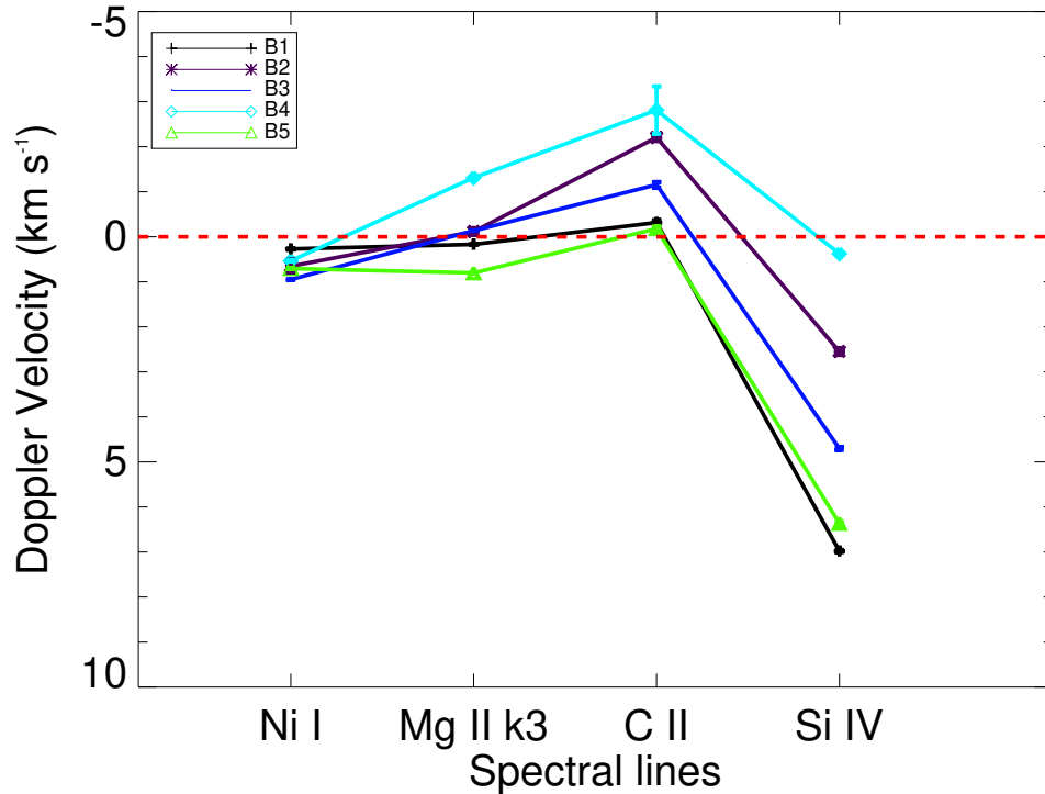
Figure 11. Average Doppler velocity variations for different spectral lines dominating at different heights in the solar atmosphere for boxes B1, B2, B3, B4, and B5 at the footpoints of quiescent coronal loops.
