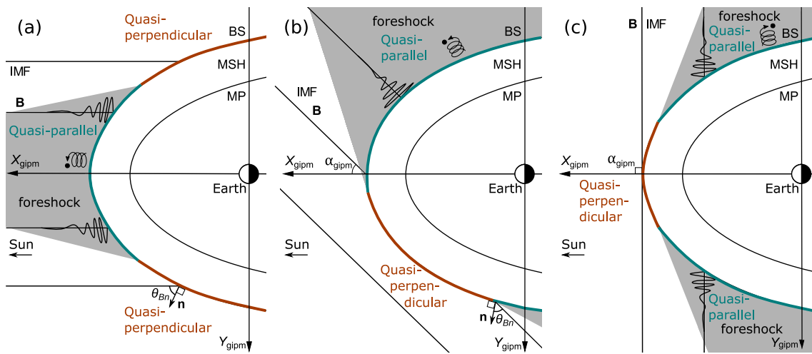
Figure 1. A sketch of the approximate foreshock regions (filled with gray) and the quasi-parallel (turquoise) and the quasi-perpendicular (brown) parts of the bow shock (BS) for IMF cone angles: (a) \alpha_{\text{gipm}} \sim 0^\circ (radial IMF) (b) \alpha_{\text{gipm}} \sim 45^\circ (e.g., Parker spiral IMF), and (c) \alpha_{\text{gipm}} \sim 90^\circ . These are presented in the plane containing the solar wind velocity vector (anti-parallel to the X_{\text{gipm}} -axis) and the IMF. The magnetopause (MP) and the magnetosheath (MSH) are shown downstream of the bow shock.
