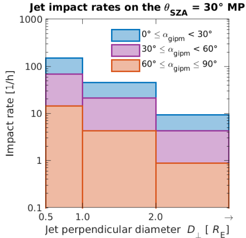
Figure 5. Estimated jet impact rates on the 30^{\circ} solar zenith angle (SZA) subsolar magnetopause as a function of jet size perpendicular to the propagation direction. The estimations are based on the model introduced by Plaschke et al. (2016).
