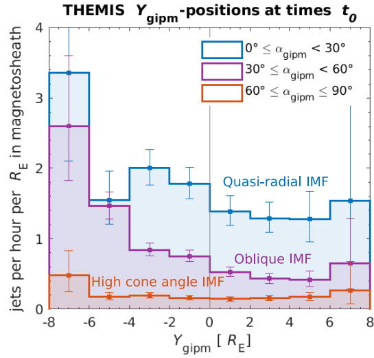
Figure 3. The number of jets observed per hour per R_E in the subsolar magnetosheath as functions of Y_{gipm} for the three cone angle ranges. The positions have been renormalized to the mean SW dynamic pressure 1.76 nPa.
