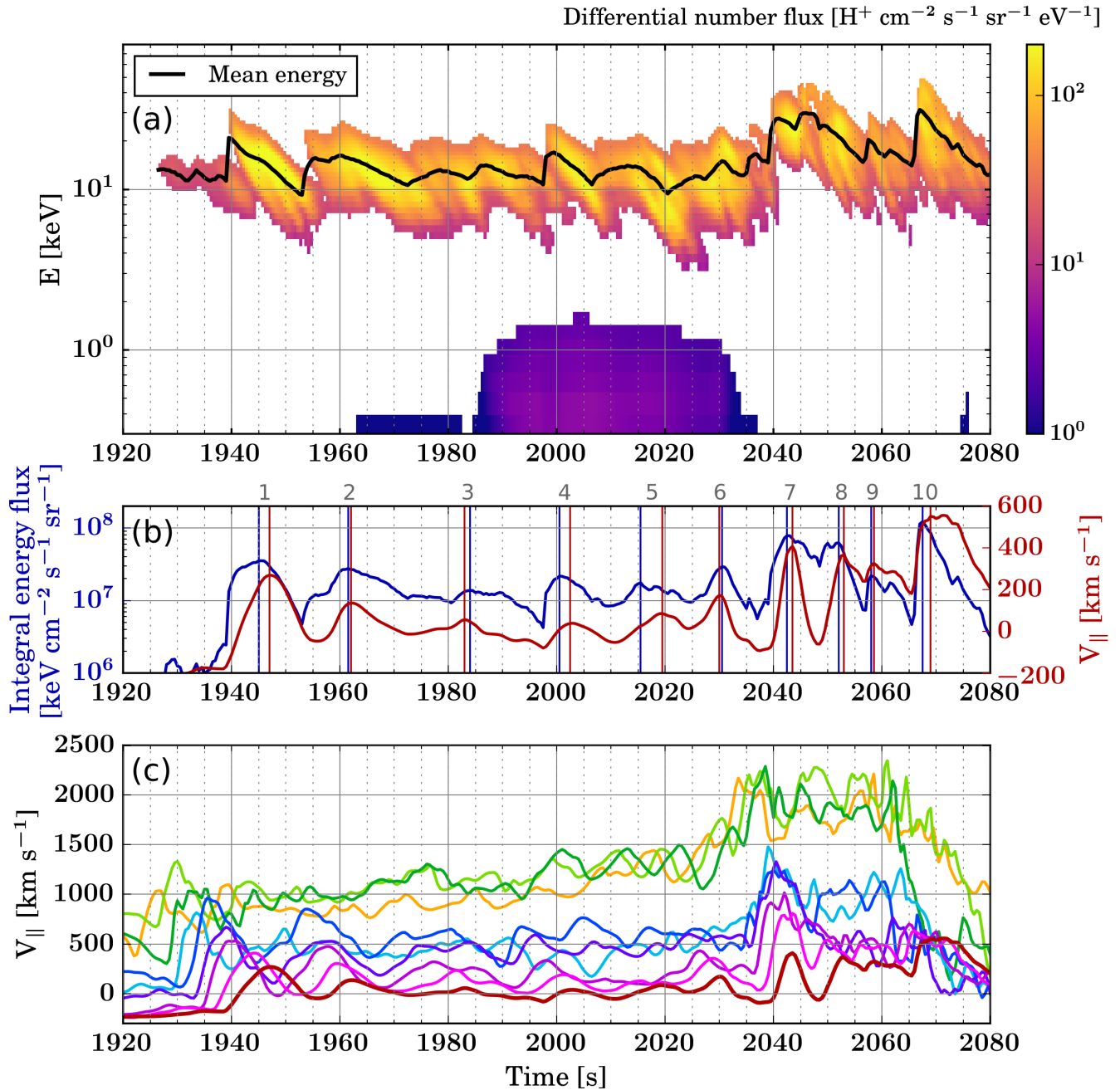
Figure 7. (a) Differential number flux of precipitating protons observed at virtual spacecraft S_1 between t = 1920 s and t = 2080 s. The black line indicates the mean precipitating energy as a function of time. (b) Blue line: Integral energy flux associated with proton precipitation as a function of time at virtual spacecraft S_1 . Red line: Parallel component of the plasma bulk velocity at S_1 . The vertical lines indicate the times associated with peak values for these two parameters, and the numbers in grey above the panel identify the precipitation bursts discussed in the text. (c) Parallel component of the plasma bulk velocity at S_1 and at the virtual spacecraft indicated with plus signs in Fig. 6, with a consistent colour code.
