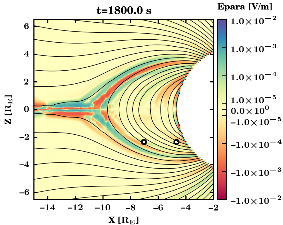
Fig. 1. Parallel electric field at t = 1800 s, averaged over 120 s
