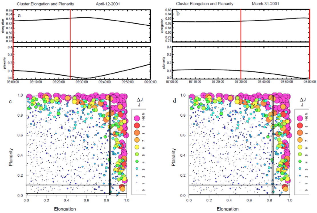
15 Figure 7: Panel a and b: Cluster elongation and planarity for two studied events. The red vertical lines demarcate the concerned time interval. Panel c and d are picked from Robert et al. (1998) to evaluate the influence of the tetrahedron shape. Black lines mark the elongation and planarity obtained from panel a and b.
