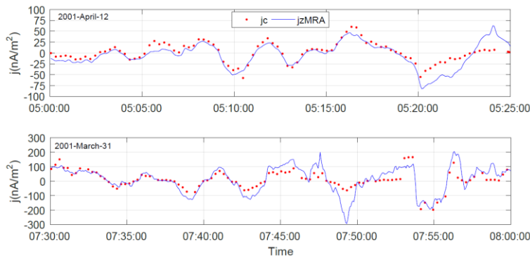
15 Figure 6: The z component current density calculated from MRA method (the blue curve) and the estimated curvature current (the red dotted curve).
