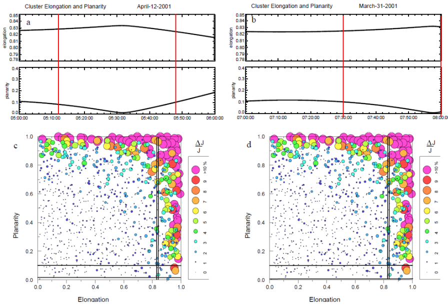
Figure 7: Panel a and b: Cluster elongation and planarity for two studied events. The red vertical lines show the concerned time interval. Panel c and d are picked from Robert et al. (1998).
