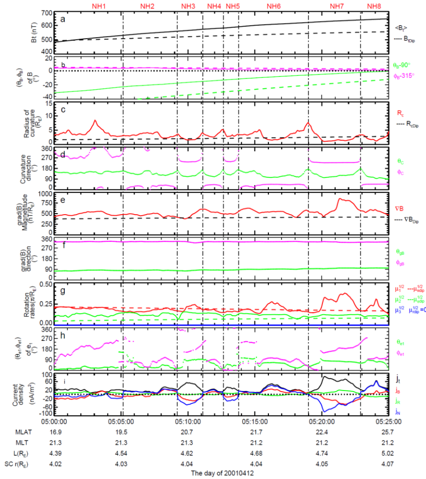
Figure 2: Geometry of the magnetic field and the current distribution in the NH region on 12 April 2001. (a) Average magnetic strength B_i at the center of the Cluster tetrahedron (black solid line) and the calculated strength B_{iDip} of the dipole geomagnetic field (black dashed line). (b) Direction angles (\theta_B, \phi_B) of the magnetic field. 90^\circ and 315^\circ are reduced respectively for \theta_B and \phi_B to better indicate the magnetic field variation. The polar angle and azimuthal angle of dipolar fields is also show in dashed lines. (c) Radius of curvature, R_c (red solid line), and the calculated radius of curvature, R_{cDip} , of the dipole geomagnetic field (black dashed line). (d) Direction angles (\theta_c, \phi_c) of the curvature of the MFLs. (e) Value of the gradient of magnetic field strength for the real magnetic field (red solid line) and dipole geomagnetic field (black dashed line). (f) Direction angles (\theta_{gB}, \phi_{gB}) of the gradient of magnetic field strength. (g) Maximum, median, and minimum rotation rates of the measured magnetic field (solid lines) and dipole geomagnetic field (dashed lines). (h) Direction angles (\theta_{e1}, \phi_{e1}) of the maximum rotation rate. (i) Total current density
