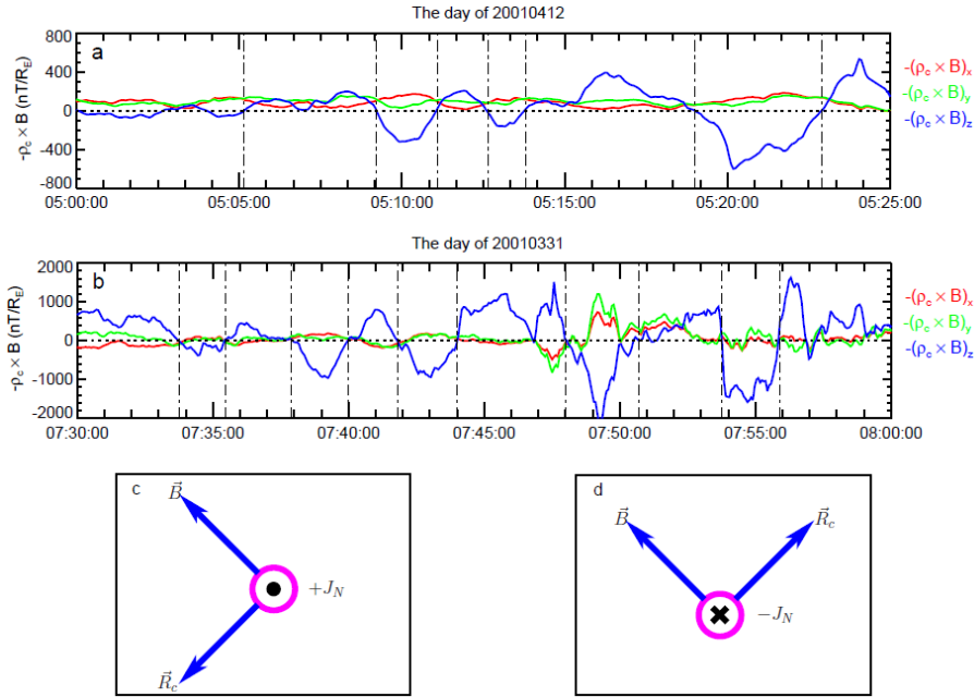
Figure 5: (a) and (b) Results deduced from the radius of curvature of the cross magnetic field. (c) and (d) Cartoon plots of the origin of the \dot{J}_N current variation.
