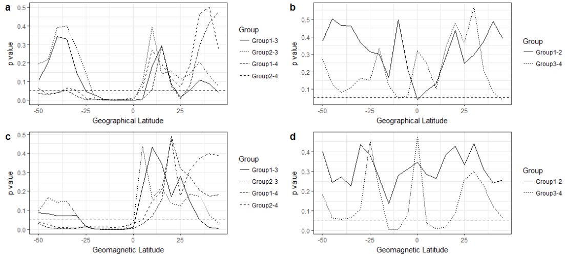
Fig. 4 Variations of p-values with geographical/ geomagnetic latitude
