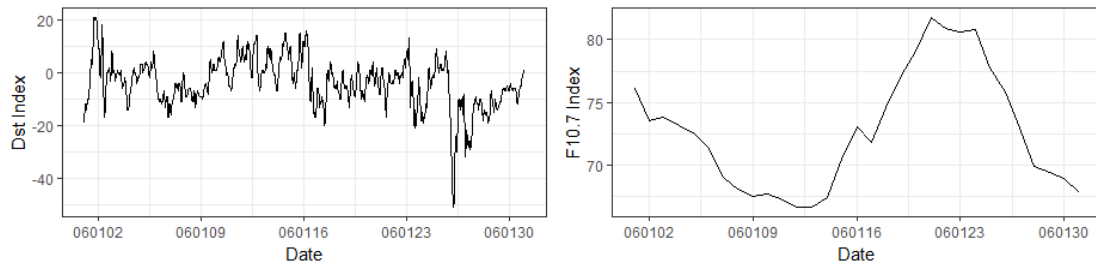
Fig. 2 Geomagnetic index Dst and solar activity index F10.7 in January 2006
