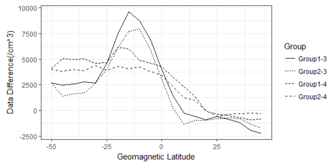
Fig. 5 Variations of data differences with geomagnetic latitude
