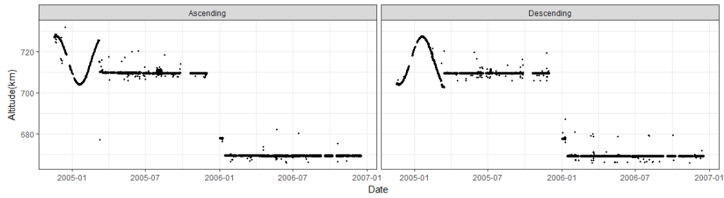
Fig. 1 Average altitude of the DEMETER satellite from November 2004 to December 2006
