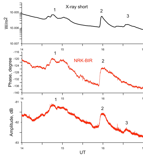
Figure 7. Fluctuations of X-ray flux for X9.3 solar flare on September 6 during the recovery phase (top panel) and phase and amplitude variations of the signal in the NRK-BIR path (temporal resolution is 1 s).
