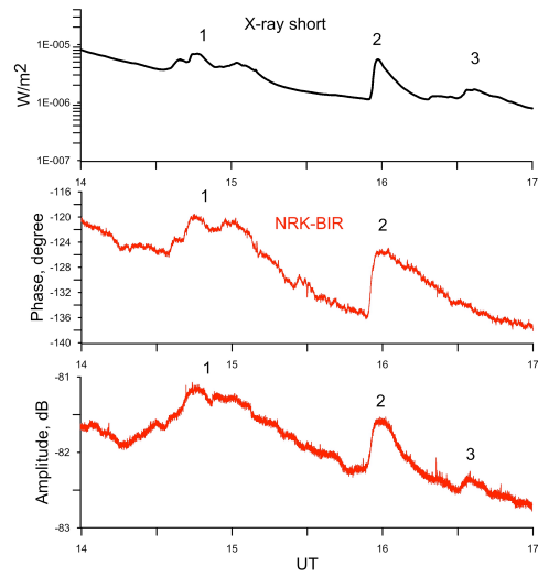
Figure 7. Fluctuations of X-ray flux for X9.3 solar flare on September 6 during the recovery phase (top panel) and phase and amplitude variations of the signal in the NRK-BIR path (temporal resolution is 1 s).
