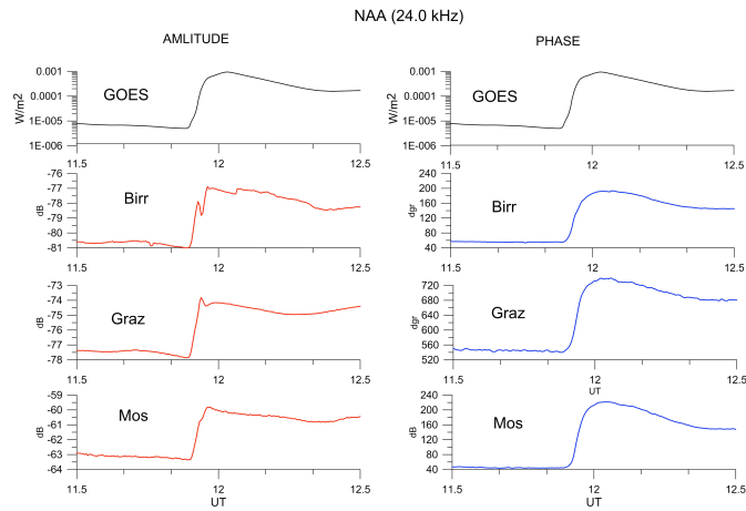
Figure 2. Amplitude (left) and phase (right) anomalies recorded in the NAA signal in Birr, Graz and Moscow receiving stations during the X-ray burst on September 6, 2017. Top panel shows X-ray flux measured with GOES satellite in the wavelength range of 0.05-0.4 nm.
