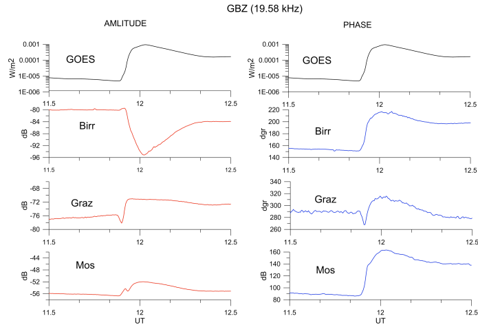
Figure 3. Same as Figure 2, but for the signal from GBZ transmitting station.
