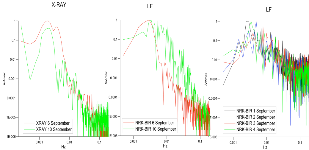
Figure 6. Spectra of X-ray and LF data (filtered in range 5 sec-16 min) for the two solar flares. The spectra of the same signal for quiet days are shown in the right panel for comparison.
