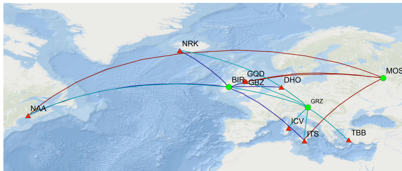
Figure 1. Positions of the receivers (green circles) in Birr, Ireland (BIR), Graz, Austria (GRZ) and Moscow, Russia (MOS) together with positions of the eight transmitters (red triangles), which have been used in this study.
