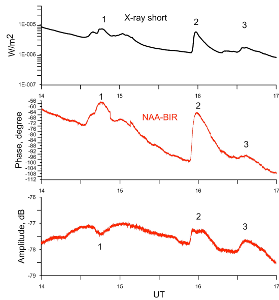
Figure 8. Same as in Figure 7 for the wave path NAA-BIR.
