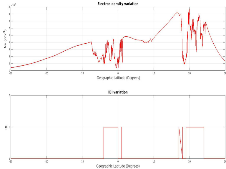
Figure 0. Swarm A electron density variations on 2014-10-06 in comparison with IBI
