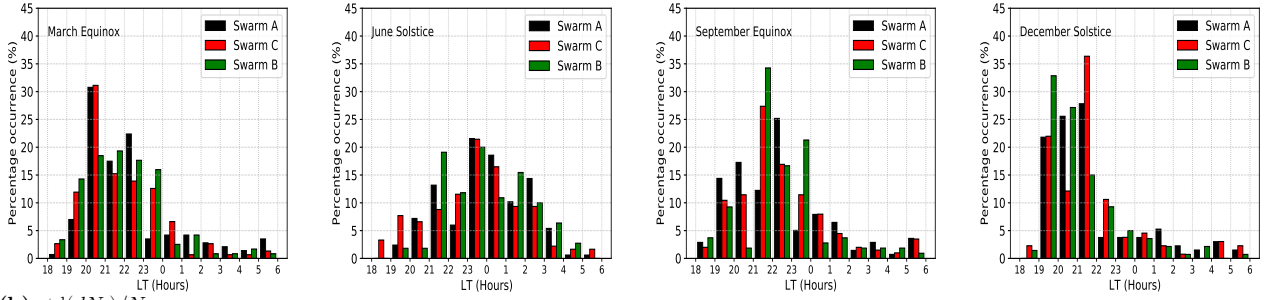
(b) \text{std}(dN_e)/N_e
