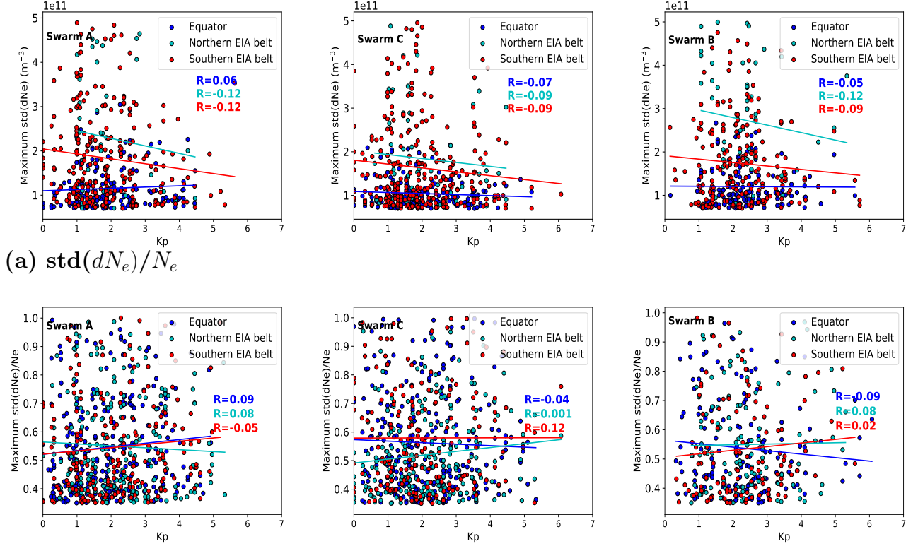
(a) \text{std}(dN_e)
