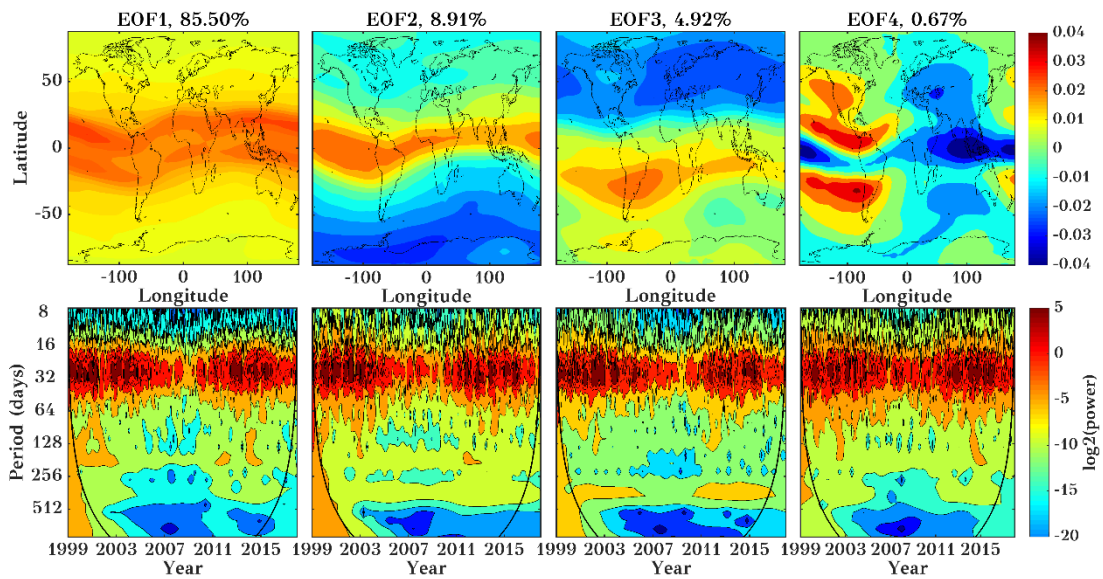
Figure 13: Spatial distribution map of first four EOFs (upper panel) of IGS TEC during the years 1999 to 2017, and their corresponding wavelet transform (lower panel, wavelet power in log2 scale) using a 25-35 days filtered datasets. The EOFs are dimensionless.
