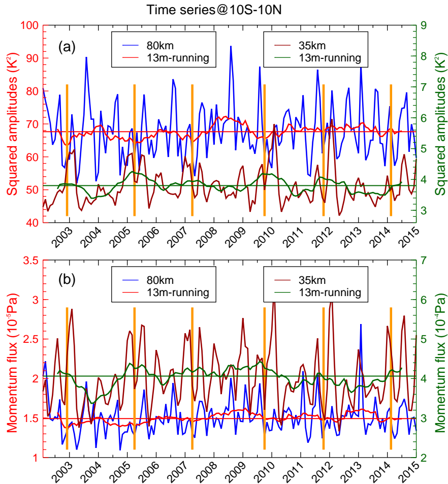
Figure 8. Time series of GW squared temperature amplitudes (a) and absolute momentum flux (b) at 80 km (blue lines) and 35 km (brown lines). Values are averaged over the latitude band 10^{\circ}S-10^{\circ}N . 13-month running means (red lines for 80 km and green lines for 35 km, respectively) are given to highlight the overall QBO signals. The horizontal red and green lines are the median values. Maxima of GW activity at 35 km are marked by orange vertical lines in order to highlight the quasi-biennial variations.
