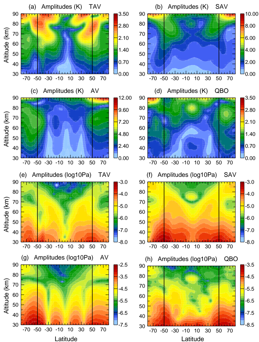
Figure 11. Altitude-latitude sections of spectral amplitudes for terannual, semiannual, annual, and QBO variation obtained by sinusoidal fits of the time series of square-root of monthly zonal mean GW square temperature amplitudes (a–d, unit in K) and GW absolute momentum flux (e–h, unit in log10(Pa)).
