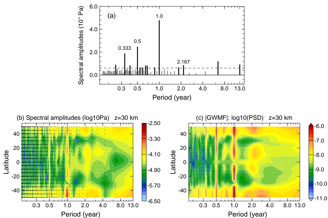
Figure 1. Example of an FFT spectrum of absolute GWMF performed at the latitude 45^{\circ}\text{N} and altitude 50 km (a), and latitude dependence of the spectra at 30 km altitude for the latitude range 50^{\circ}\text{S} – 50^{\circ}\text{N} (b). For comparison, also the MEM spectra at 30 km altitude are displayed for the latitude range 50^{\circ}\text{S} – 50^{\circ}\text{N} (c). The significance level of 1.3 times the average spectral amplitude is shown as a horizontal dashed line in (a). Black dots in (b) indicate spectral amplitudes below the significance level of 1.3 times the average spectral amplitude.
