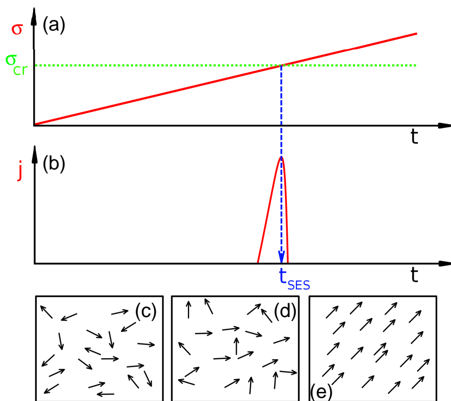
Figure 2. Schematic diagram of the condensed matter physical model proposed for the SES generation. (a) Before an EQ, the stress \sigma gradually increases in the focal area versus the time t towards reaching a critical value \sigma_{cr} . (b) When \sigma reaches \sigma_{cr} a transient electric signal is emitted that constitutes an SES. (c) Random orientation of the electric dipoles at small stress. (d) Partial orientation at an intermediate stress \sigma < \sigma_{cr} . (e) Cooperative orientation of the electric dipoles when \sigma = \sigma_{cr} .
