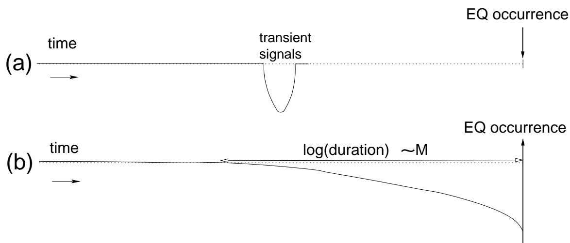
Figure 1. Schematic diagram showing the two distinct approaches proposed for a precursory behavior. (a): The case of the condensed matter physical model for SES generation, which differs greatly from other suggested mechanisms (Rikitake, 1981) in which the anomalous precursory behavior becomes more intense upon approaching the EQ occurrence (b).
