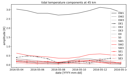
Figure 12. Tidal temperature modes at 45 km altitude from global MERRA-2 fields at the latitude of 54° N.
