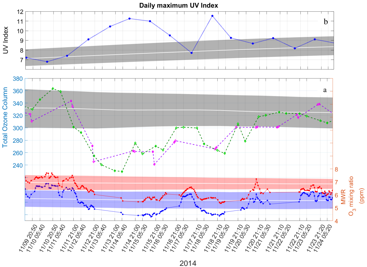
5 10 15 Figure 7. Atypical event of Antarctic ozone hole influence over Río Gallegos. (a) (Bottom) Time evolution a of the MWR ozone mixing ratio at 27 km (red line) and 37 km (blue lines). Light red and light blue areas represent the ozone mixing ratio zonal climatology at both altitudes calculated using MLS database (2004 - 2016). (Top) Time evolution of total ozone column measured with the ground-based SAOZ instruments (green dots) and OMI (purple dots) in Dobson Units. White line and grey area represent the climatology and one SD calculated using the OMI data-base (2004 - 2017). (b) Time Evolution of the Daily maximum Ultraviolet Index measured with the ground-based solar radiometer YES UVB-1 at OAPA. White line and grey area represent the climatological UVI at noon in Río Gallegos.
