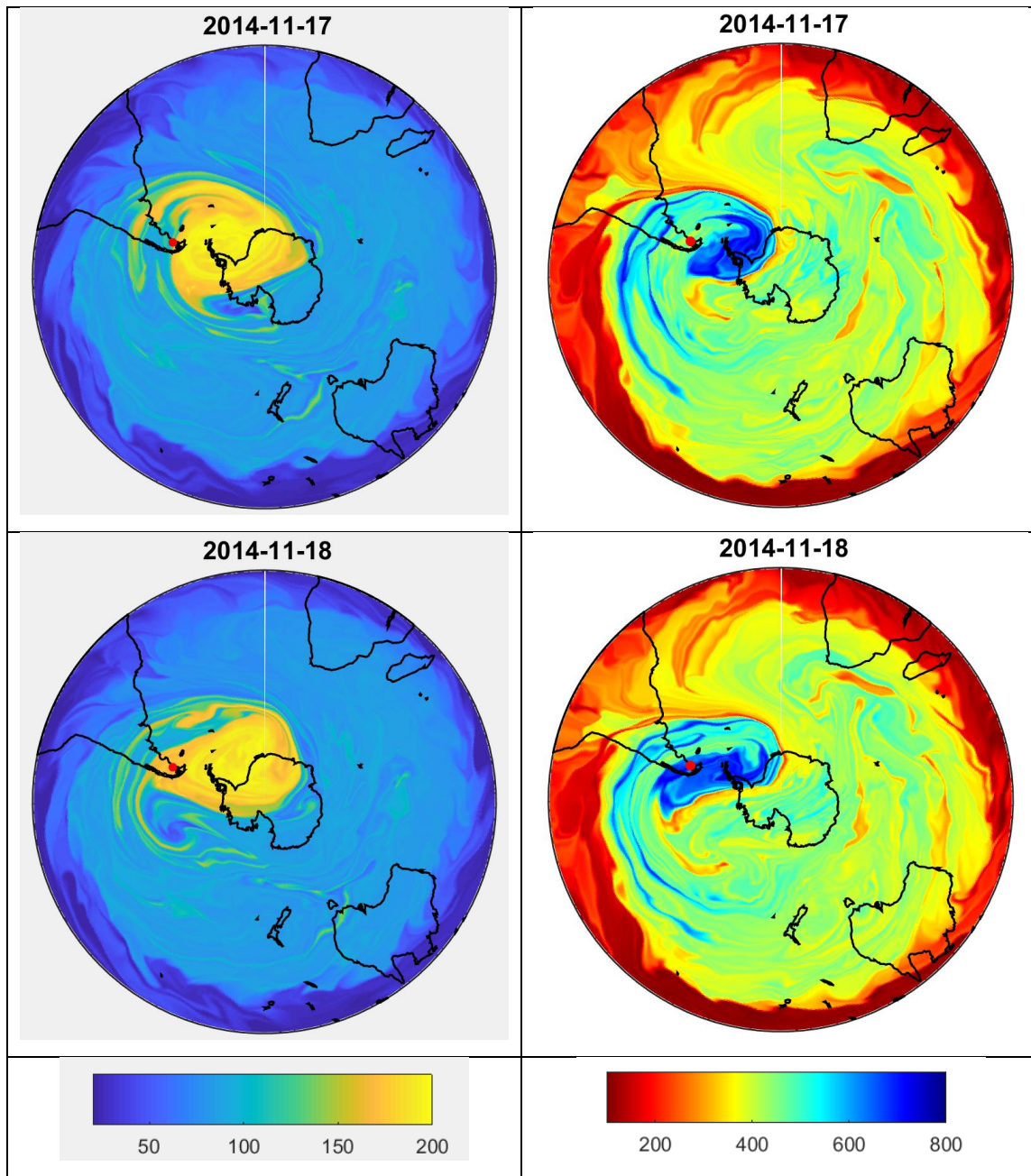
Figure 8 Advected Potential Vorticity maps assimilated with the MIMOSA model. Maps show the evolution of the polar vortex for two isentropic levels with potential temperatures of 675K (left) and 950K (right).
