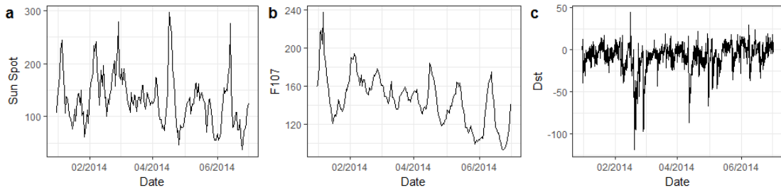
Fig. 2 Variations of solar and geomagnetic indices with time
