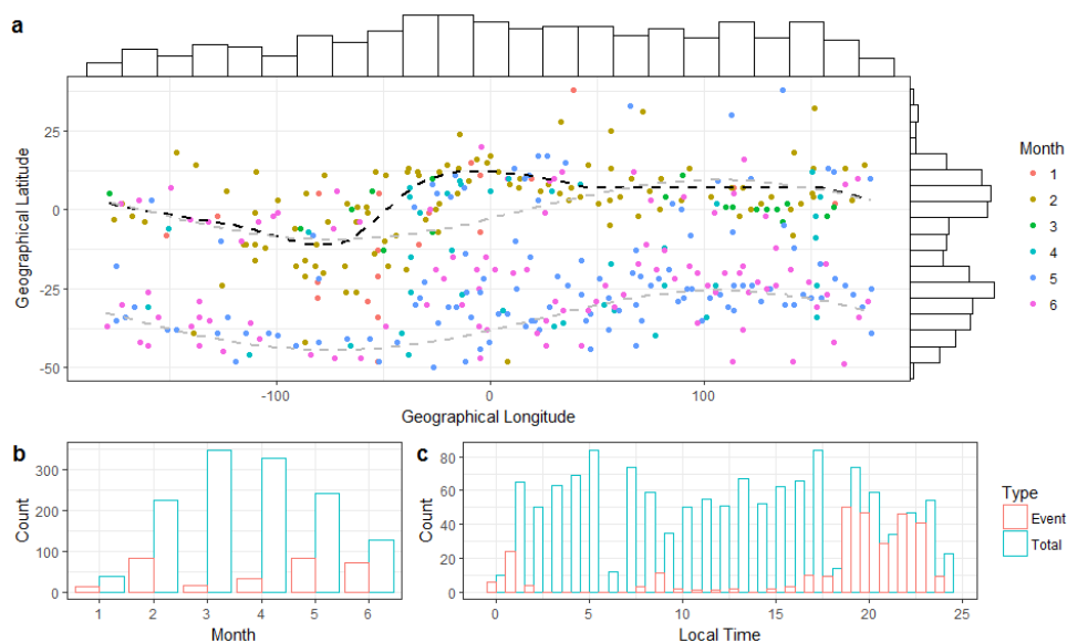
Fig. 3 Distribution of detected stratification events and variations of occurrence number with local time and month
