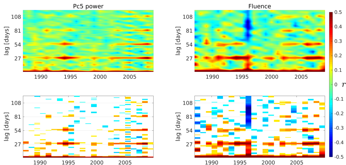
Figure 5. Two dimensional plots of ACFs of every year. In the abscissa axis is the year and in the ordinate axis is the lag (between 0 and 120 days). The top-left(top-right) panel shows the Pc5 power(fluence) ACFs with the neighboring values interpolated. White bins in the bottom panels belong to |r| values that do not exceed |CVC| .
