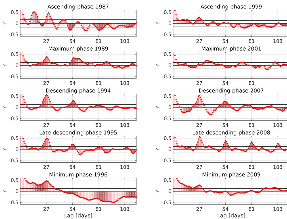
Figure 4. ACFs of electron fluence for different phases of the SC 22 (left panels) and 23 (right panels) as a function of lag in days. The horizontal black lines are the critical values of correlation.
