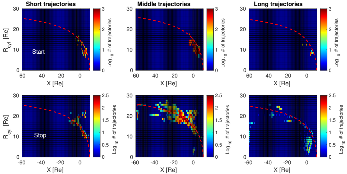
Figure 5. Cylindrical coordinates of the starting and ending positions of the launched O^+ ions depending on the length of their trajectory (see definitions in the text). The upper panels show the starting positions, while the lower panels show the ending positions. The colour bar represents the number of trajectories in each bin. The red dashed line shows to the average magnetopause for the corresponding events.
