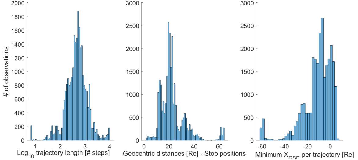
Figure 4. (a) Length of the 26200 O^+ trajectories in our sample. Note the logarithmic scale. (b) Final positions expressed in the geocentric distance R given in Re (see text for definition). (c) Minimum X distance for each trajectory.
