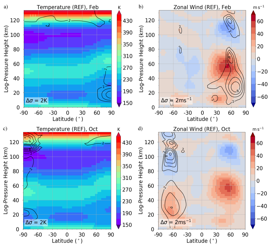
Figure 2. (a,c) REF zonal mean temperature and (b,d) zonal wind. (a-b) February conditions. (c-d) October conditions. Results are an average of 11 ensemble members (shaded color). Standard deviations \sigma are 2 K for temperature and 2 \text{ms}^{-1} for zonal wind.
