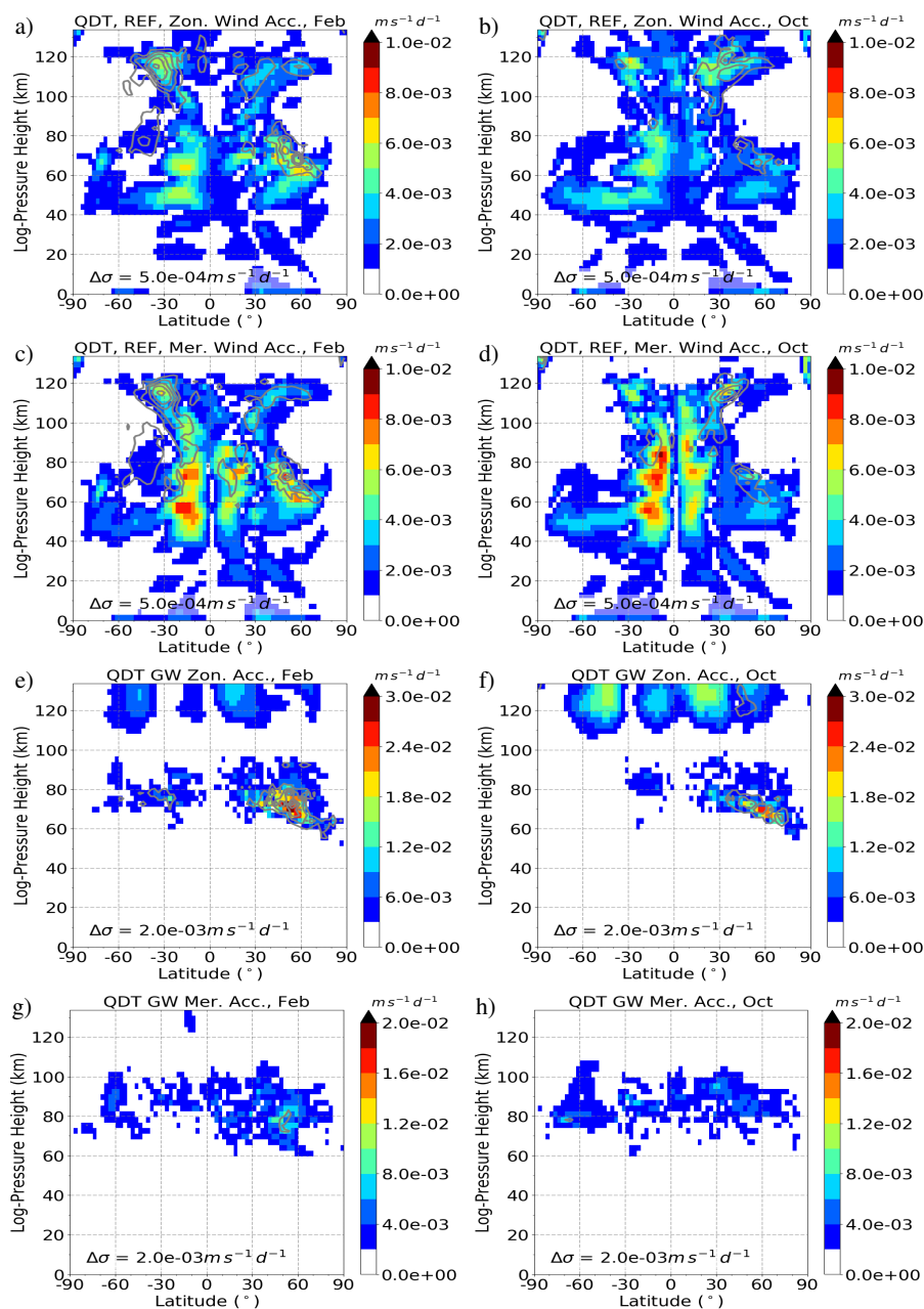
Figure 4. Quarterdiurnal component of zonal and meridional wind acceleration terms in the REF simulation for February conditions (a, c, e, g) and October conditions (b, d, f, h). Amplitudes are scaled by \exp[-z(2H)^{-1}] . Results are an average of the 11 ensemble members (shaded color). Standard deviations ( \sigma ) are added as grey contour lines. (a, b) zonal wind advection (nonlinear component), (c, d) meridional wind advection (nonlinear component), (e, f) zonal and (g, h) meridional acceleration due to GWs (tendency terms from GW parameterization). Note that the color scales are different.
