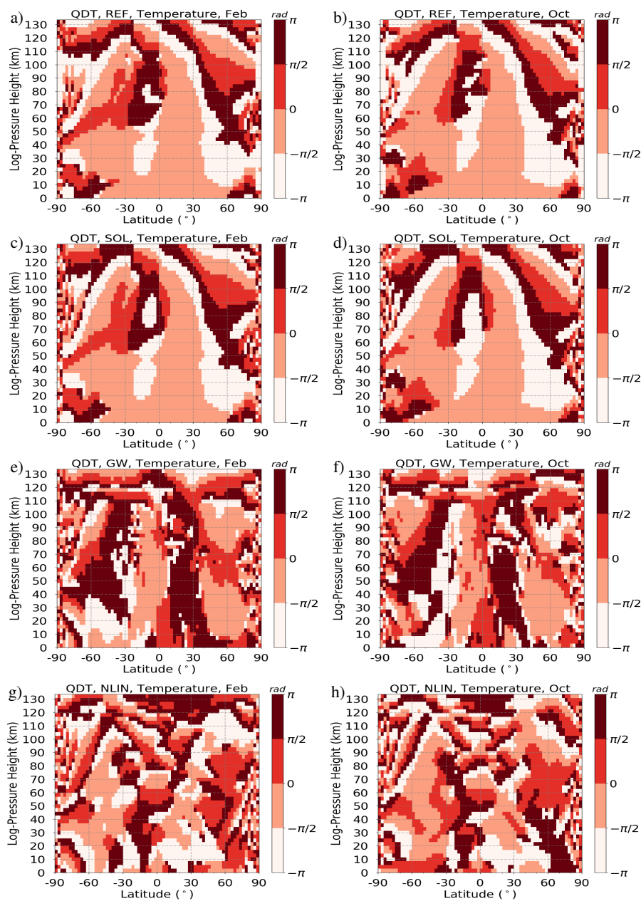
Figure 6. Simulations of zonal mean QDT phases for temperature (colors). (a, c, e, g) February and (b, d, f, h) October conditions. (a, b) REF run with all forcing mechanisms enabled, (c, d) SOL run with just direct solar forcing mechanism enabled, (e, f) GW run with just GW forcing mechanism enabled and (g, h) NLIN run with just nonlinear forcing mechanism enabled. Standard deviations \sigma are added as gray contour lines.
