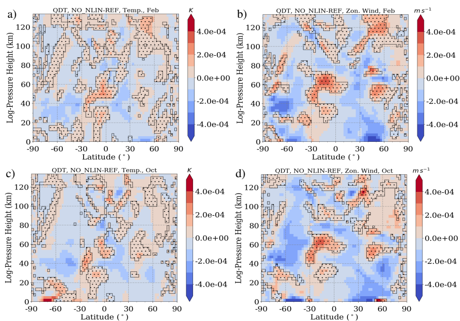
Figure 9. Difference of QDT amplitudes between NO_NLIN and REF simulation, scaled by \exp[-z(2H)^{-1}] . Red colors denote larger NO_NLIN simulation amplitudes and blue colors denote larger REF simulation amplitudes. Areas of destructive interference ( 120^\circ \leq \Delta\Phi \leq 240^\circ ) between NLIN and SOL phases are hatched. (a, c) temperature, (b,d) zonal wind. (a, b) February conditions. (c, d) October conditions.
