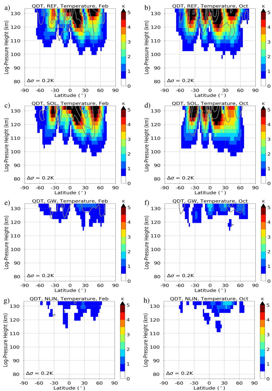
Figure 5. Simulations of zonal mean QDT amplitudes for temperature (colors). (a, c, e, g) February and (b, d, f, h) October conditions. (a, b) REF run with all forcing mechanisms enabled, (c, d) SOL run with just direct solar forcing mechanism enabled, (e, f) GW run with just GW forcing mechanism enabled and (g, h) NLIN run with just nonlinear forcing mechanism enabled. Standard deviations \sigma are added as gray contour lines.
