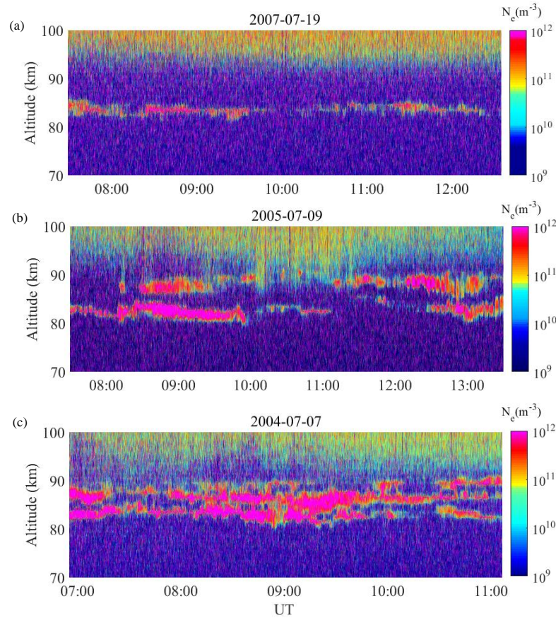
5 Fig. 1 The typical layered PMSE events observed by EISCAT 224MHz VHF radar. a) The observation on 19 July, 2007 (Upper panel) Monolayer PMSE ; b) The observation on 9 July, 2005 (Middle panel) Double layer PMSE ; c) The observation on 7 July, 2004 (lower panel) Tri-layer PMSE . The red circle marks the obvious layered phenomenon of PMSE events.
