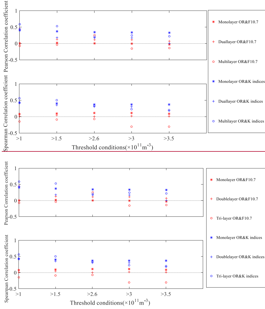
Fig. 9 Pearson linear and Spearman rank correlation computed between layered PMSE OR (with threshold conditions of N_e \geq 1 \times 10^{11} \text{m}^{-3} , N_e \geq 1.5 \times 10^{11} \text{m}^{-3} , N_e \geq 2.6 \times 10^{11} \text{m}^{-3} , N_e \geq 3 \times 10^{11} \text{m}^{-3} and N_e \geq 3.5 \times 10^{11} \text{m}^{-3} , respectively) and F_{10.7} corresponding to the occurrence of PMSE and between layered PMSE OR and K index corresponding to the occurrence of PMSE, respectively. For each correlation coefficient, P value is less than 0.05. The horizontal dotted line is drawn to separate positive and negative correlation coefficients.
