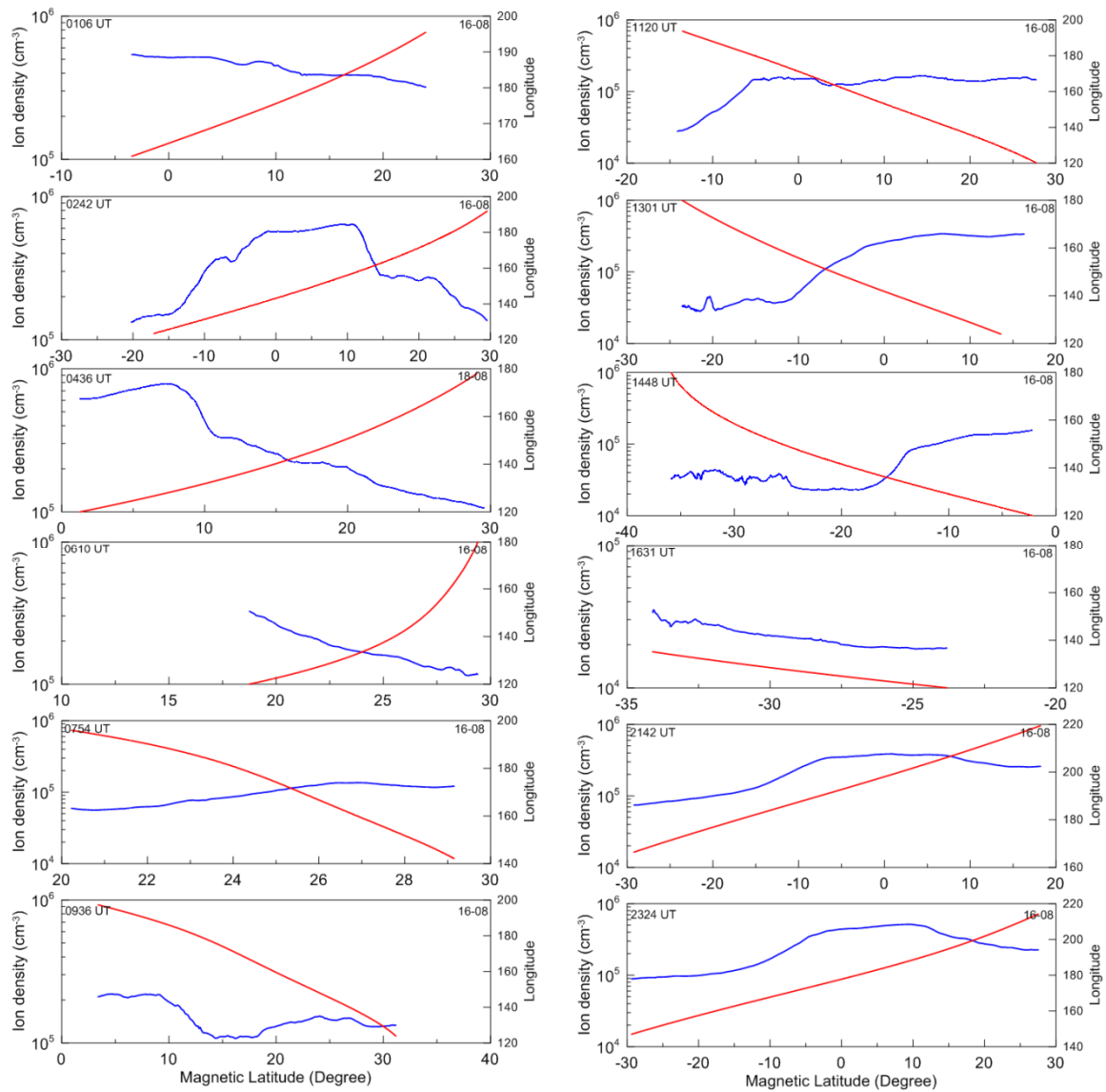
Figure 1. Variations of ion densities and longitudinal tracks along the ROCSAT-1 trajectories during successive times on 16 August in 170°E region
