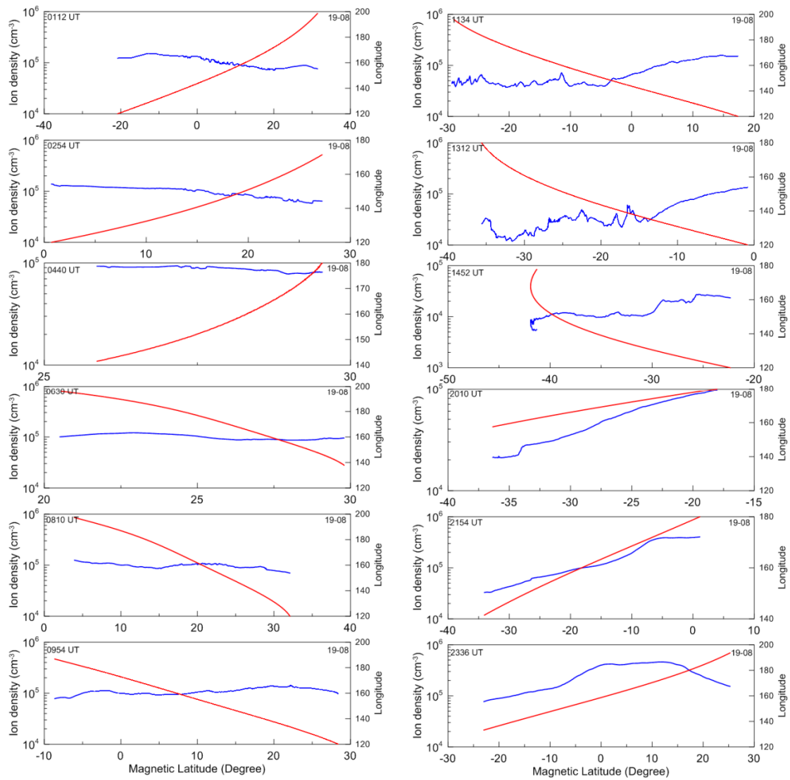
Figure 2. Variations of ion densities and longitudinal tracks along the ROCSAT-1 trajectories during successive times on 19 August in 170°E region
