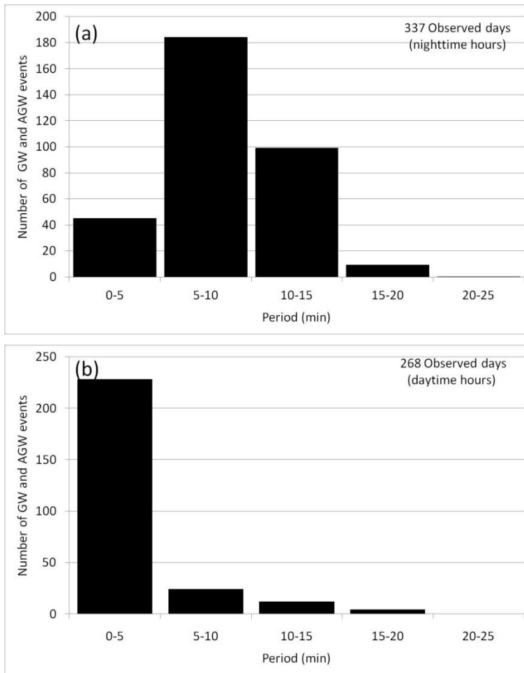
Figure 7: Histogram plot of the predominant observed wave periods of the GWs detected in the low ionosphere as amplitude variations of the VLF signal propagating in the NAA-EACF GCP. Histogram plots of the predominant observed wave periods of the small-scale AGWs detected in the lower portion of the ionosphere as amplitude variations of the VLF signal propagating in the NAA-EACF during night (a) and day (b) hours.
