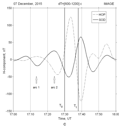
Figure 9. Wave “portrait” of polar substorms: (a) variations of H-component in a band 15 \pm 5 min along meridian, the presumable width of auroral oval is indicated with gray; (b) latitudinal distribution of pulsation intensity; (c) out-of-phase variations at stations SOD and HOP where latitudinal distribution of pulsation intensity has maxima. Open arrows indicate time of enhancement of pre-breakup arcs. T_0 and T_1 are the times of onset and torch formation, respectively.
