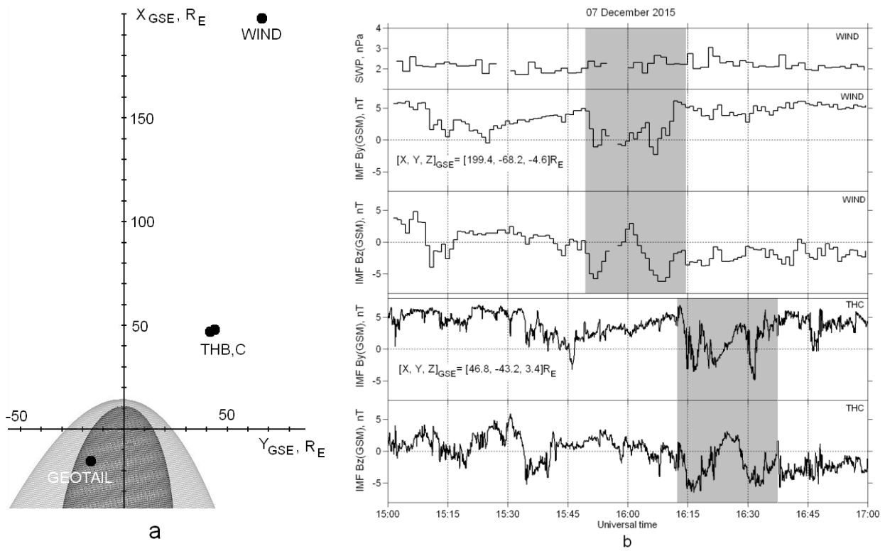
Figure 6. (a) satellite positions in solar wind (WIND, THB and THC) and in the magnetosphere (GEOTAIL); (b) variations of the solar wind pressure and IMF Bz and By components. Two negative excursions of Bz on the both satellites resembling the quasi-sinusoidal variation with period \sim 15 min are highlighted by gray.
