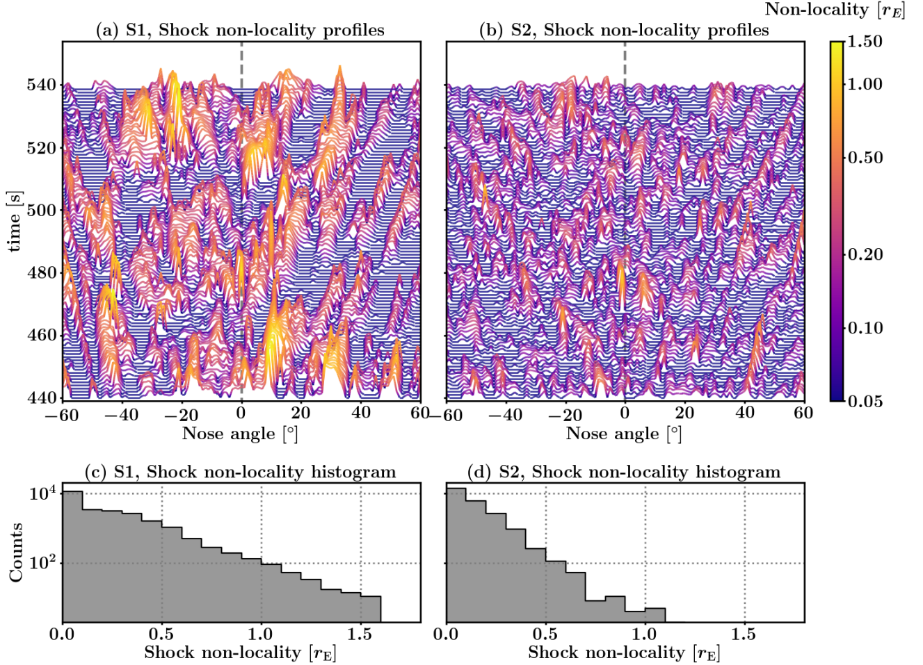
Figure 3. Panels (a) and (b): profiles of measured shock non-locality as a function of nose angle for simulations S1 and S2, respectively. The y -axis indicates simulation time, used as the base level corresponding with a well-defined shock with a non-locality measure of zero. Regions of enhanced non-locality are shown as colored peaks of the curve, as presented in the color bar. A dashed vertical line indicates nose angle 0^\circ . (a): S1. (b): S2. Both plots show chains of enhanced non-locality regions, which move away from the nose region and decrease in intensity as they approach the flanks. Under each stacked profile plot we show a histogram depicting the occurrence rate of different non-locality values, with panel (c) depicting S1 and panel (d) depicting S2.
