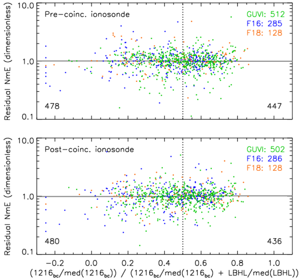
370 Figure 3: Residual NmE (y-axis, as described in the text) plotted versus the ratio of background-corrected 1216 to the sum of background-corrected 1216 and LBHL, where the radiances are normalized by their medians. The upper and lower panels show results for ionosonde observations immediately before and after (respectively) the times of satellite coincidence with the ground stations. Horizontal gray lines indicate the median residual values in left and right bins on either side of the dotted vertical line at x=0.5 . The numbers of points in the bins are displayed in the lower left and right corners of the panels. The numbers of points shown for each satellite are given in the upper right corners of the two panels.
