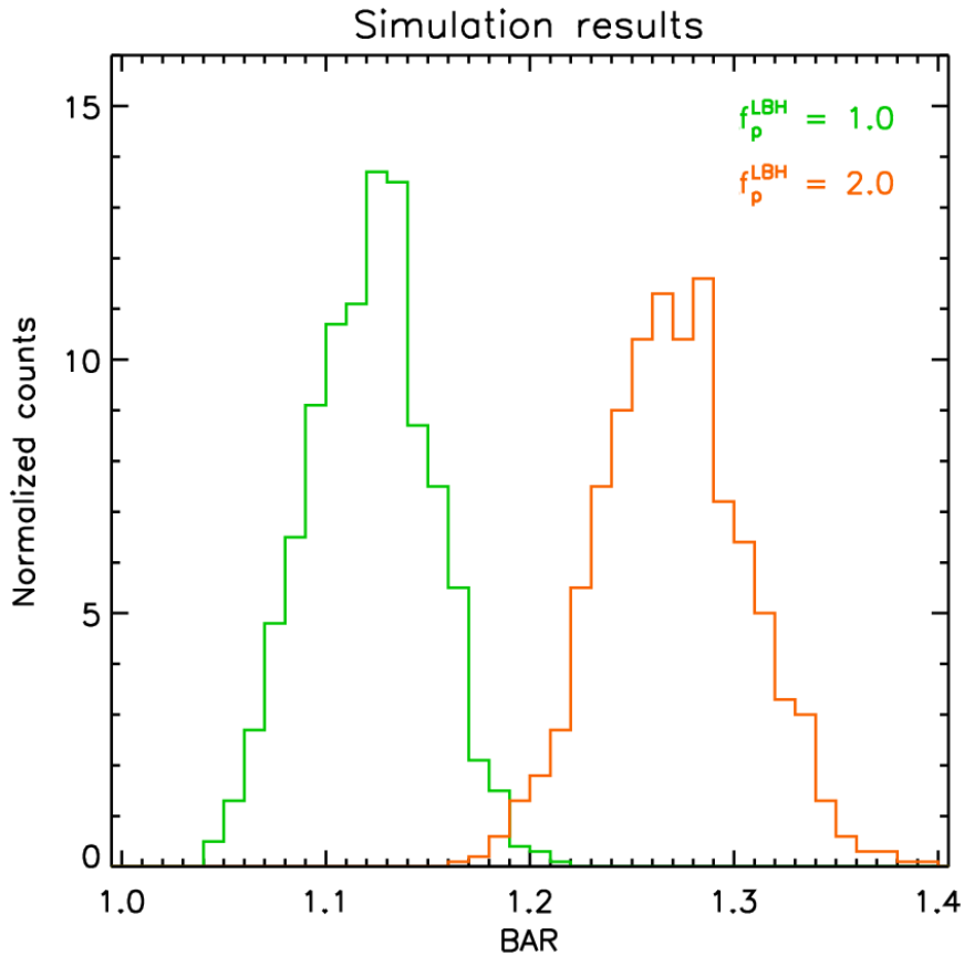
550 Figure A1: Histograms of below-to-above ratios (BAR, defined in Section 4.1) from 1000 randomized simulation runs (each) for f_p^{\text{LBH}} = 1.0 (green) and f_p^{\text{LBH}} = 2.0 (orange). The counts (i.e., numbers of BAR statistics that fall in each histogram bin) are normalized so that the integrated area under each curve equals unity.
