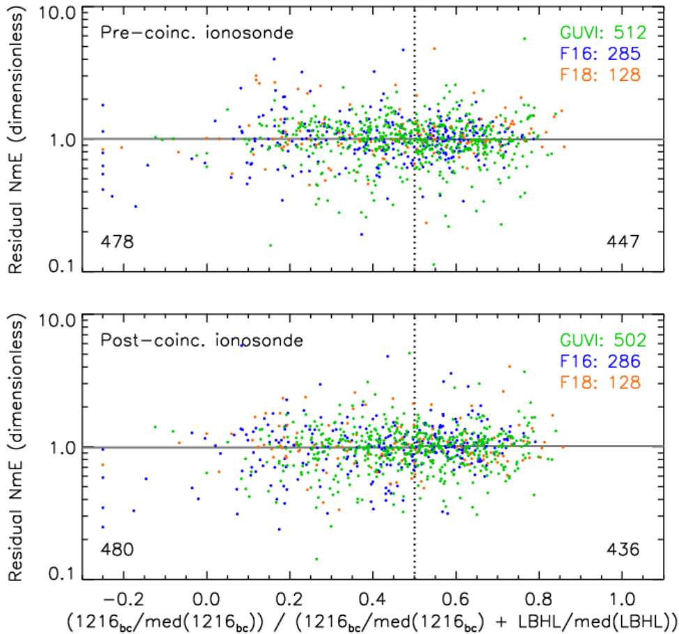
360 Figure 3: Residual NmE (y-axis, as described in the text) plotted versus the ratio of background-corrected 1216 to the sum of background-corrected 1216 and LBHL, where the radiances are normalized by their medians. The upper and lower panels show results for ionosonde observations immediately before and after (respectively) the times of satellite coincidence with the ground stations. Horizontal gray lines indicate the median residual values in left and right bins on either side of the dotted vertical line at x=0.5 . The numbers of points in the bins are displayed in the lower left and right corners of the panels. The numbers of points shown for each satellite are given in the upper right corners of the two panels.
