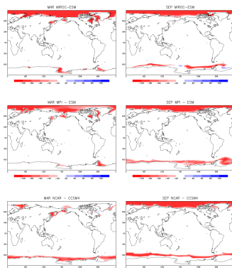
Figure 3. Sea ice concentration for the last 30 years of abrupt4CO 2 numerical experiment minus the last 30 years of the pControl run for the following models: BESM-OA V2.5, NCAR-CCSM4, GFDL-ESM4R, MPI-ESM4R, CSIRO-ACCESS, IPSL, and MIROC-ESM in March (left column) and September (right column).
