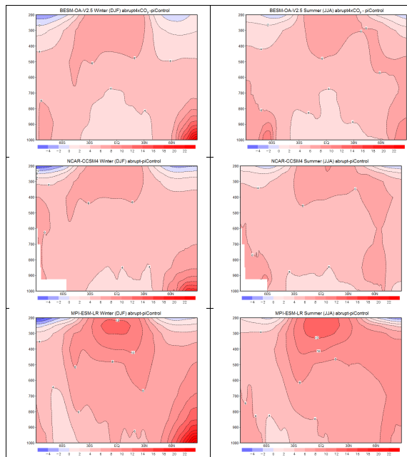
Figure 5. Zonal-average atmosphere temperature changes, in °C (Abrupt 4xCO 2 minus piControl) at each pressure level, in mb (solid line) for the last 30 years run for (a) BESM OA V2.5, (b) NCAR-CCSM4 and (c) MPI-ESM-LR model, in DJF (left) and JJA (right) columns.
